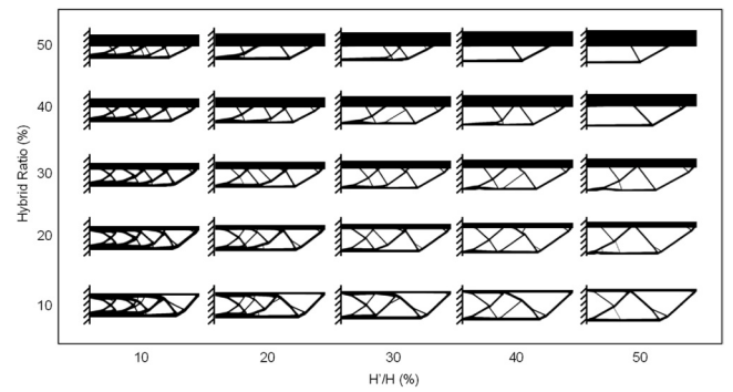
Fig. 7. Hybrid cantilever beams with identical stiffness but different H'/H and hybrid ratios.
