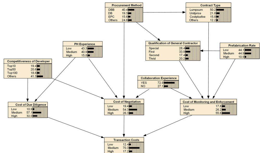
Figure 4. Bayesian Belief Network model of TCs in Chinese PH projects.
