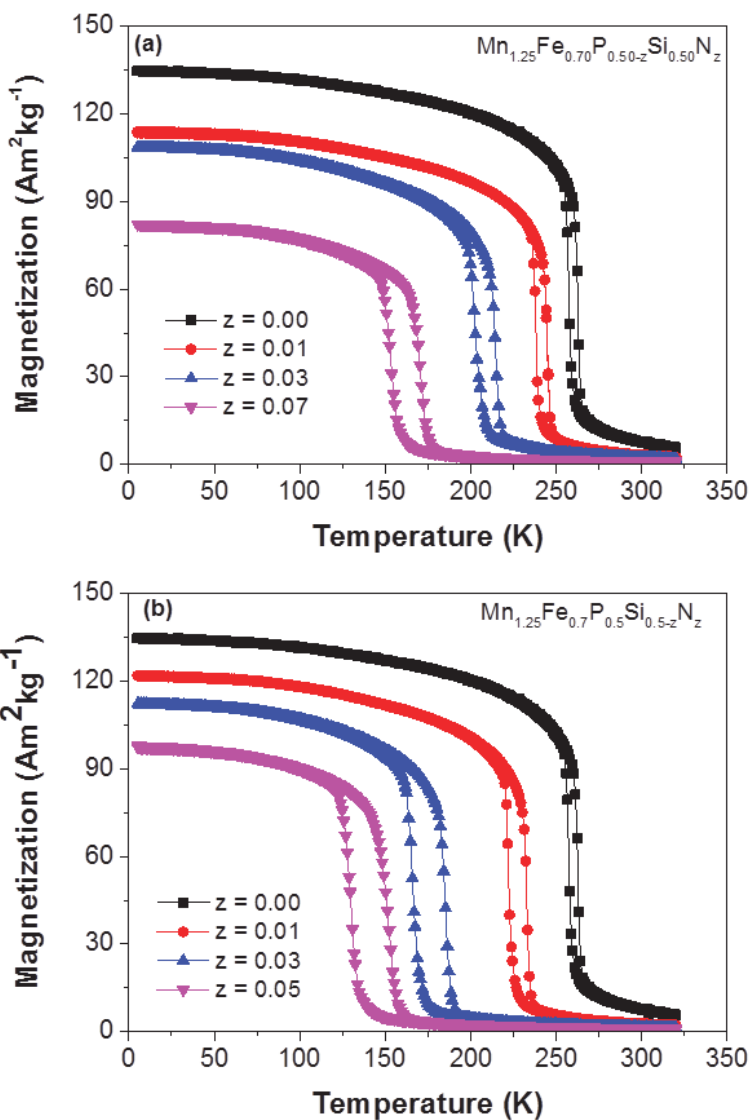
Figure 6.8: Magnetization curves measured on heating and cooling in a magnetic field of 1 T for the \text{Mn}_{1.25}\text{Fe}_{0.70}\text{P}_{0.5-z}\text{Si}_{0.5}\text{N}_z (a) and \text{Mn}_{1.25}\text{Fe}_{0.70}\text{P}_{0.5}\text{Si}_{0.5-z}\text{N}_z (b) compounds.
