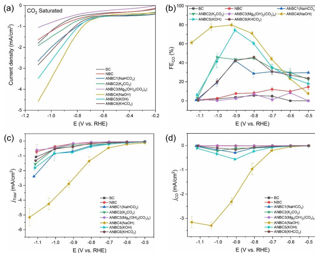
Figure 4. (a) LSV curves recorded at a scan rate of 5 \text{ mVs}^{-1} of all catalysts in a \text{CO}_2 -saturated 0.1 \text{ M KHCO}_3 electrolyte; (b) FE of CO production at applied potentials from -0.50 to -1.15 \text{ V vs. RHE} ; (c) Total current density of all catalysts at different applied potentials; (d) Partial current density of CO of all catalysts at different applied potentials.
