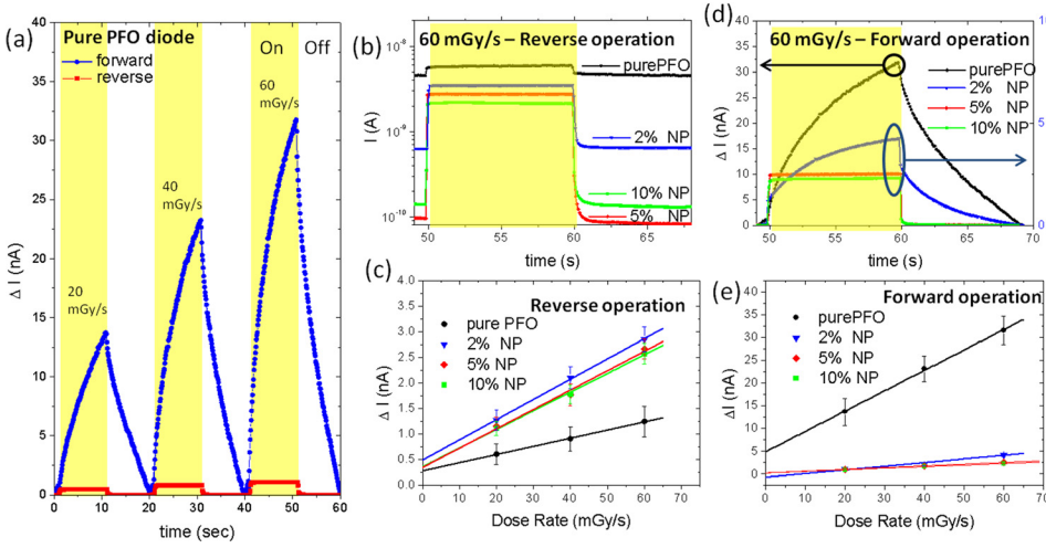
FIG. 2. X-ray detection with pure and NP-blended polymer diodes. (a) Characteristic X-ray photocurrents in a 1 \mu m thick pure PFO diode. The dark currents have been subtracted for comparison. (b) Impact of NPs on diode detector properties in reverse bias. (c) Photocurrent against the dose-rate for diodes operated in reverse bias. NP blended diodes show the largest X-ray sensitivity. (d) Impact of NPs on diode photocurrent response in forward bias. (e) Photocurrent against the dose-rate for diodes operated in forward bias. Photocurrents of the pure PFO diode increase by more than one order of magnitude with respect to reverse operation.
