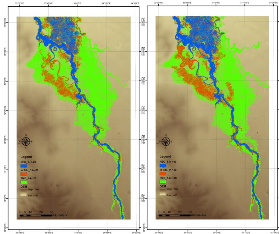
Figure 3 Comparison of flood extents of 1-in-20 year (left panel) and 1-in-100 year (right panel) return period: REC, PMC and In situ
