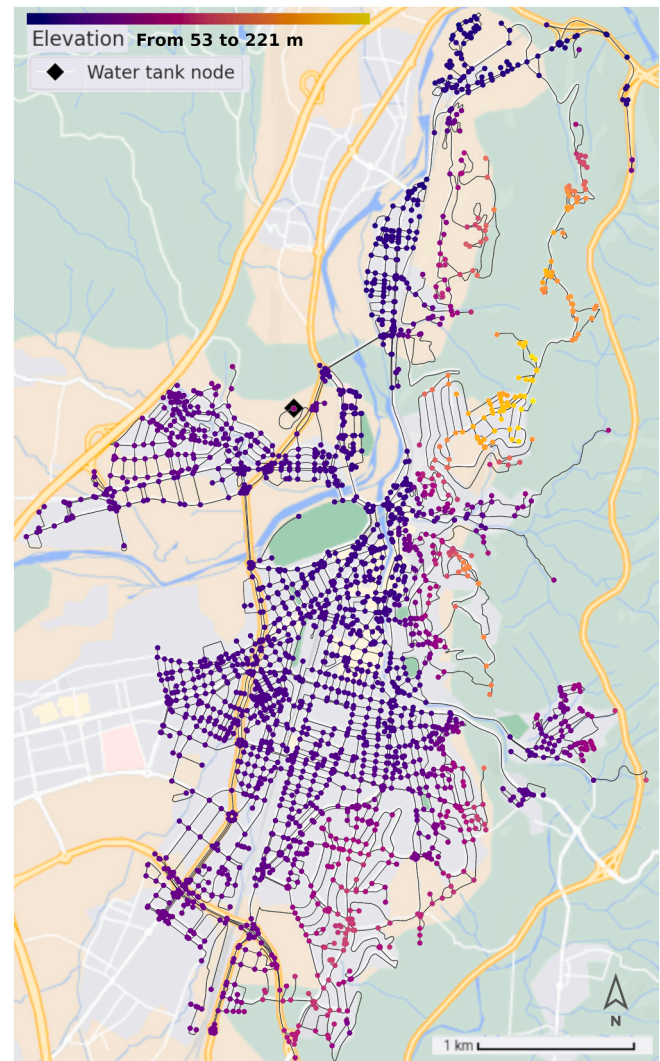
Fig. 1. Visualization of the Girona case study area, highlighting nodes color-coded by elevation, and indicating the placement of the initial water tank.
