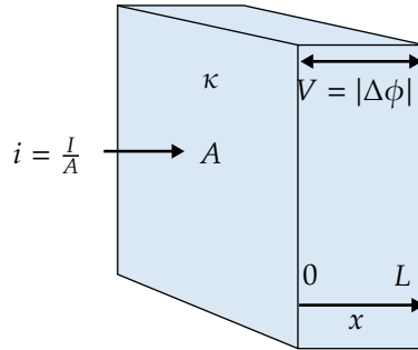
Figure 1.1: A schematic to illustrate Ohm's law V = IR and Pouillet's law R = L/\kappa A in a planar domain with ion conductivity \kappa .
