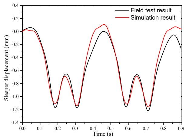
Fig. 18 (Color) Sleeper displacement results
