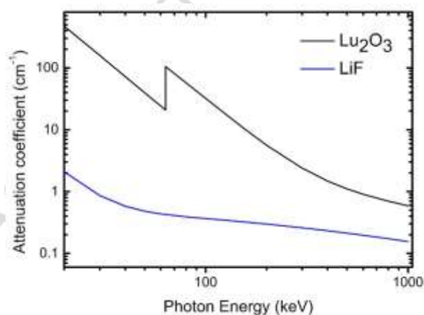
Fig. 2. Attenuation coefficients of \text{LiF} and \text{Lu}_2\text{O}_3 in the range of 20-1000 keV of energy. \text{LiF} shows very similar response to the broad range of energies of ionizing radiation, while \text{Lu}_2\text{O}_3 highly preferentially accumulates energy of the less energetic particles.
