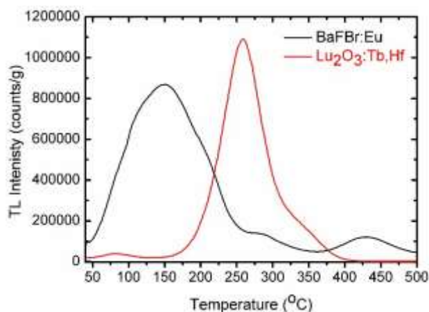
Fig. 7. Comparison of the thermoluminescence of \text{Lu}_2\text{O}_3:\text{Tb,Hf} and a commercial \text{BaFBr}:\text{Eu} . Intensity of the former reaches 65 % of the commercial storage phosphor TL. No correction for the temperature quenching (see below) was applied.
