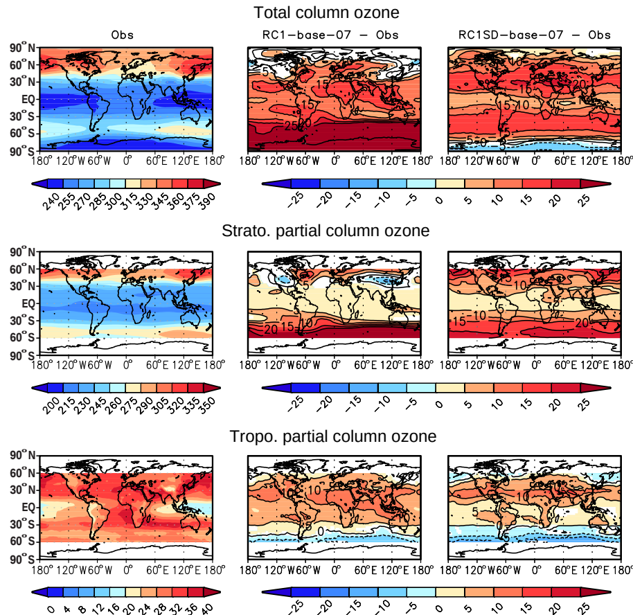
Figure 29. Left column: climatological annual mean of observed total column ozone (BSTCO, top) as well as stratospheric (middle) and tropospheric (bottom) partial column ozone (AURA MLS/OMI), all in DU. The tropospheric and stratospheric partial columns are integrated from the surface to the (on-line diagnosed, see text) tropopause and above the tropopause, respectively. The analyses cover the years 2005 to 2011. Middle column: differences between the RC1-base-07 simulation and the observations. Right column: same as middle column, but for the RC1SD-base-07 simulation. Statistically significant changes on the 95 % confidence level are coloured.
