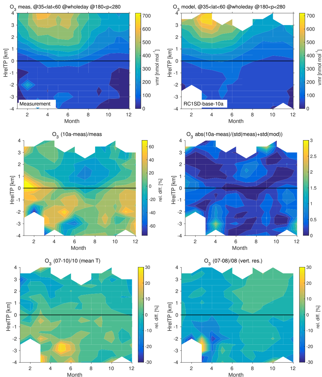
Figure 19. Comparison of O_3 climatologies ( 35\text{--}60^\circ\text{N} ) based on data from the years 2005–2013. The first row shows climatologies of CARIBIC measurements (left) and RC1SD-base-10a model data (right). The second row shows the relative differences of model data and measurements (left), and the absolute values of model minus measurements over the sum of the standard deviation of measurements and model (right). The bottom row shows the relative differences of RC1SD-base-07 and RC1SD-base-10, differing in nudging of global mean temperatures (left), and the relative differences of RC1SD-base-07 and RC1SD-base-08, with different vertical resolutions (right). The vertical axis shows the distance (in km) relative to the tropopause.
