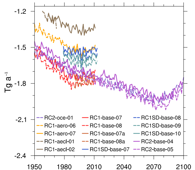
Figure 7. Simulated annual total flux of \text{CH}_3\text{OH} (in \text{Tg(C) a}^{-1} ) between atmosphere and ocean. The negative sign indicates a net uptake by the ocean.
