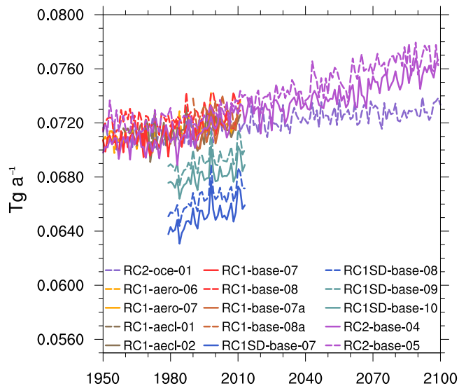
Figure 6. Simulated annual total emissions of isoprene (in \text{Tg(C) a}^{-1} ) from the ocean.
