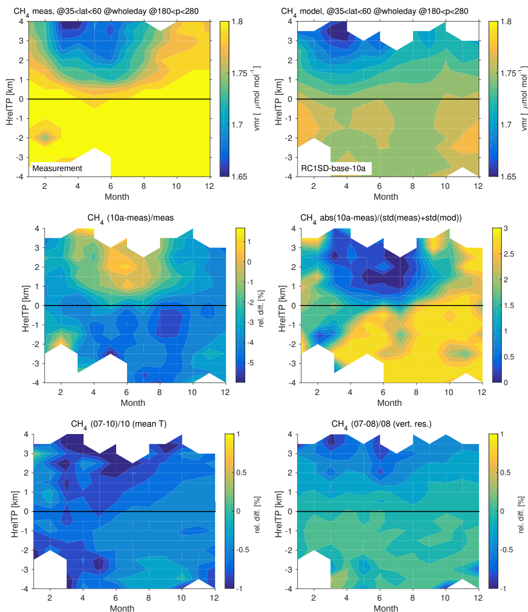
Figure 21. As Fig. 19, but for \text{CH}_4 .
