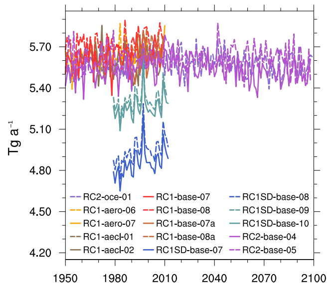
Figure 8. Simulated annual total emissions of Br from sea salt (in \text{Tg(Br) a}^{-1} ).
