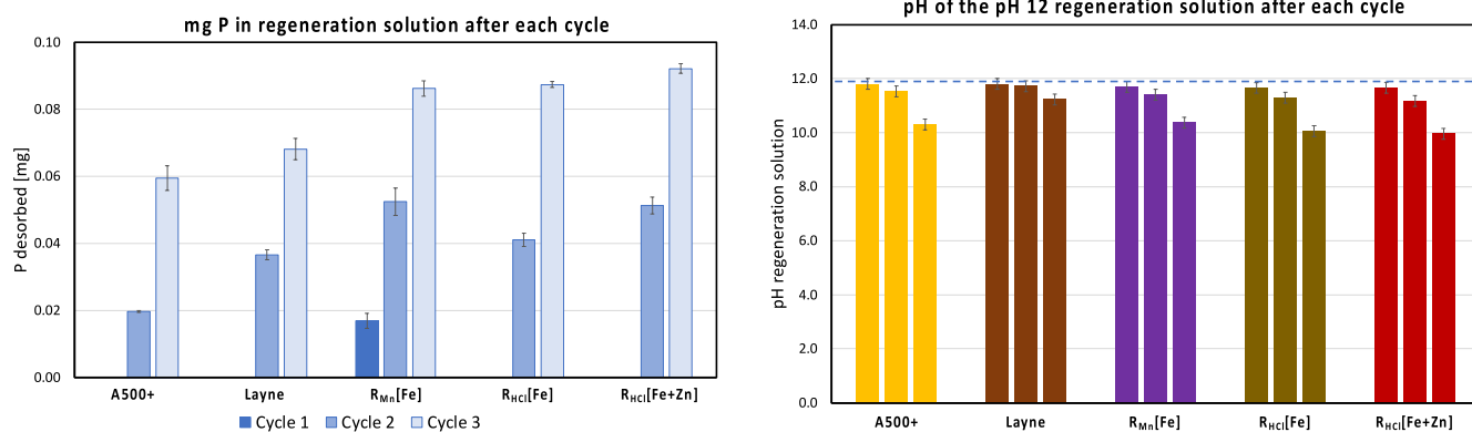
Fig. 8. P desorbed after each adsorption cycle in P-spiked wastewater, with respect to the total cumulative P loading (left); and pH value of the regeneration solution after each desorption (right), with the dashed line representing the initial pH.
