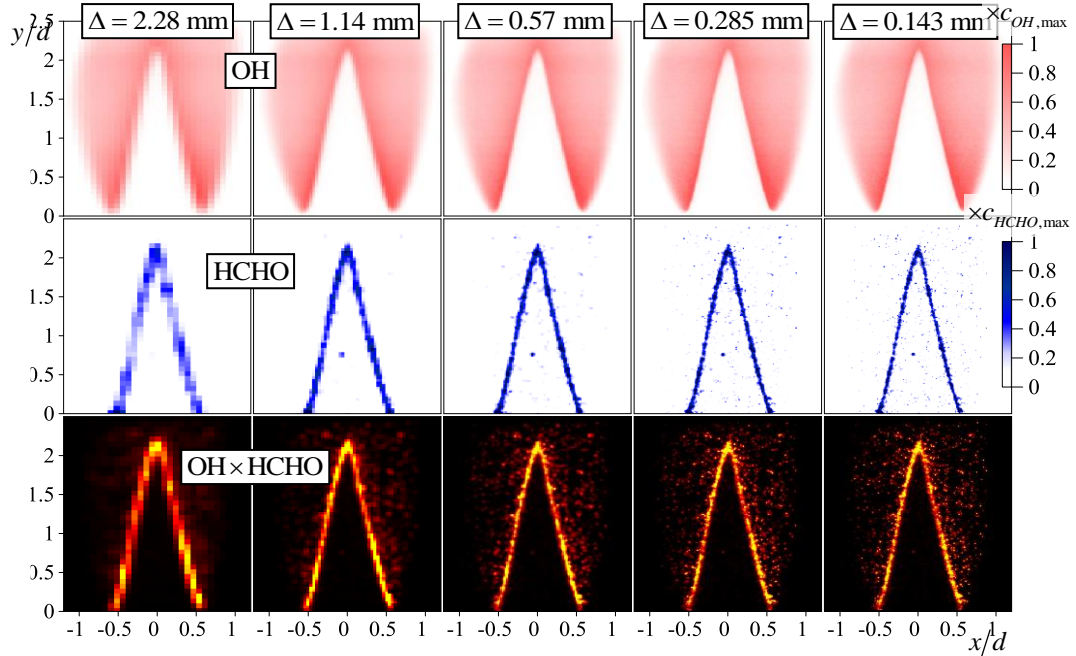
Fig. B1. Effect of the spatial resolution ( \Delta is the window size) on the instantaneous snapshots of the PLIF data for the Bunsen flame. c_{HCHO,max} = 1830 , c_{OH,max} = 31800 .
