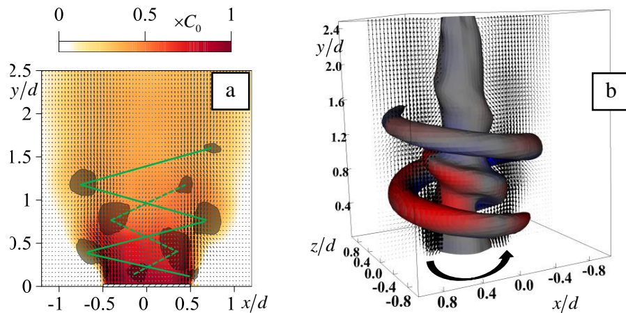
Fig. 9 Phase-averaged velocity and large-scale vortex structures in the non-reacting swirling jet.
