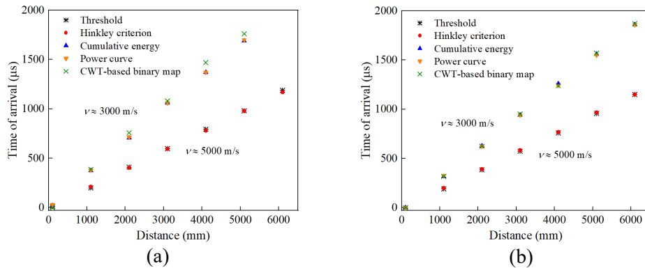
Fig. 11: Onset time versus distance curves excited at E1: (a) Test results; (b) FE model
