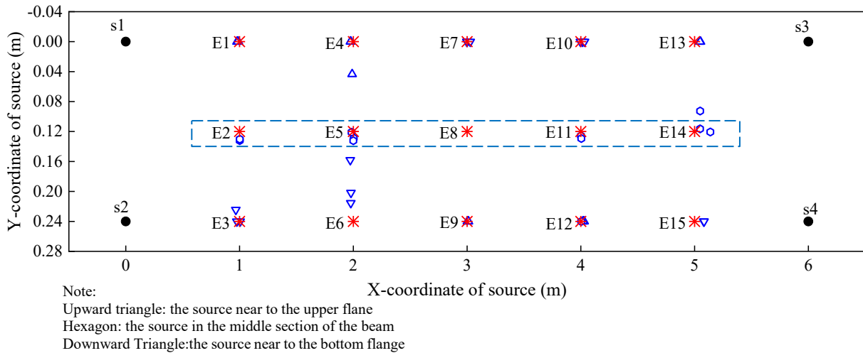
Fig. 3: Source location results
