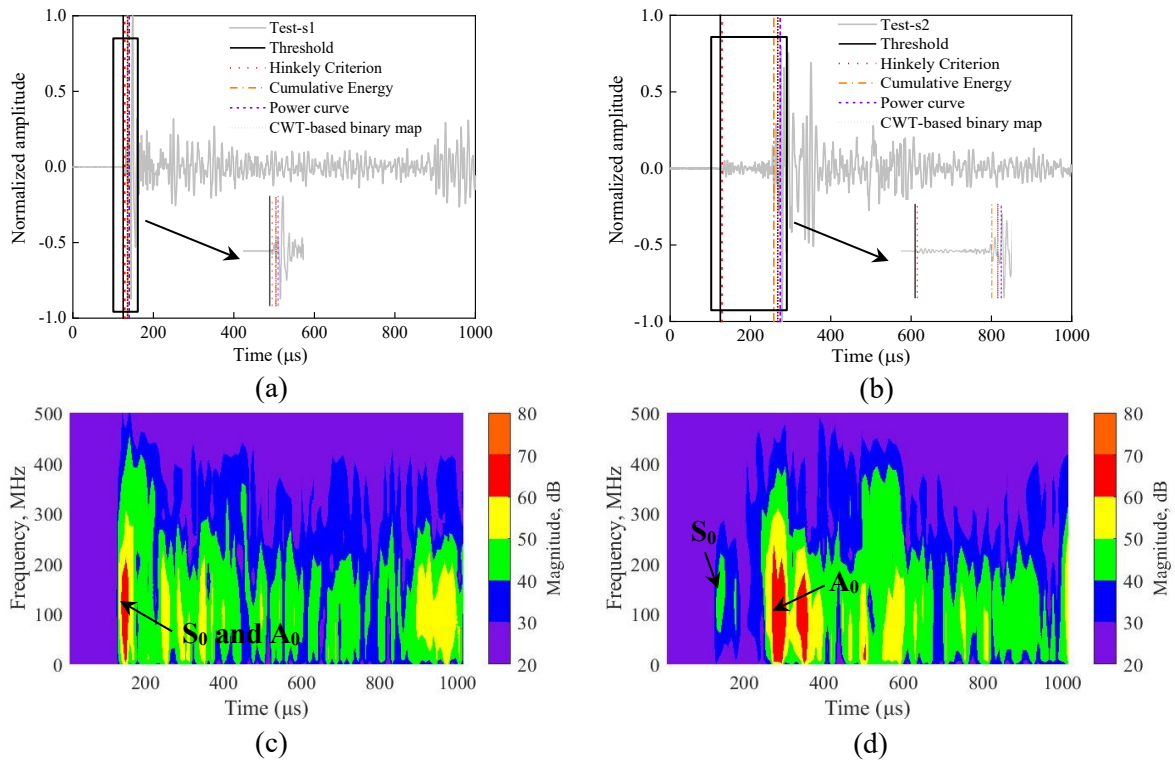
Fig. 8: Onset detection using selected methods of linear array obtained from tests: signals at (a) sensor 1 and (b) sensor 2; Amplitude spectrogram of signals at (c) sensor 1 and (d) sensor 2
