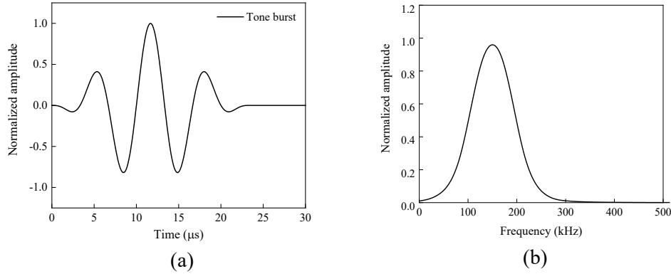
Fig. 4: The waveform used to generate signals: (a) time domain and (b) frequency domain
