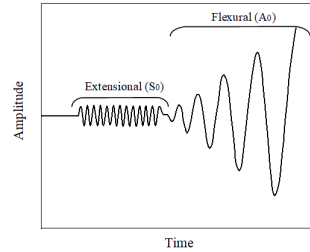
Fig. 10: Basic wave modes: Extensional ( S_0 ) and Flexural ( A_0 )
