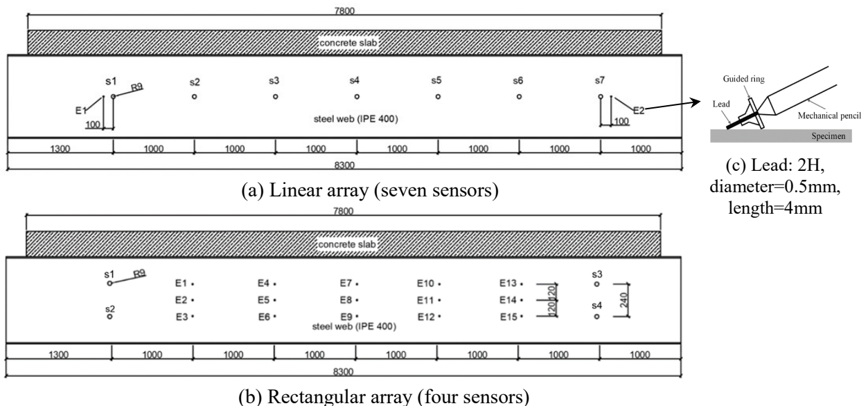
Fig. 2: Measurement setup including source location and sensor layout: Schematic view
