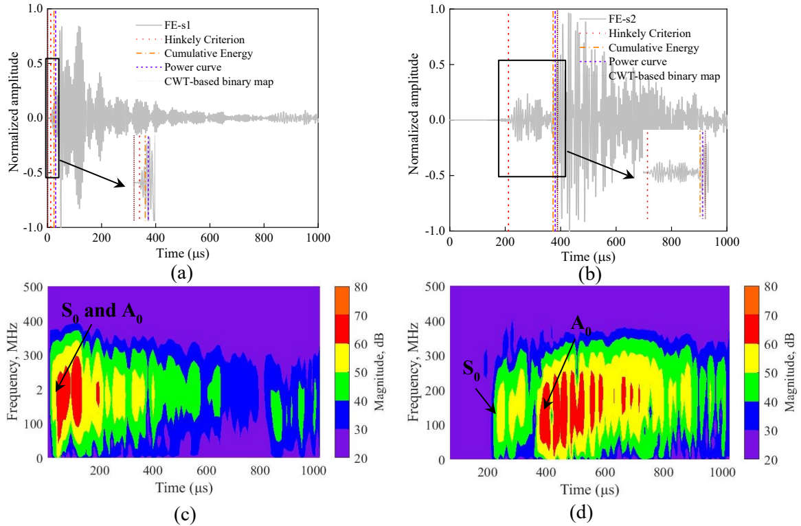
Fig. 9: Onset detection using selected methods of linear array obtained from FE model: signals at (a) sensor 1 and (b) sensor 2; Amplitude spectrogram of signals at (c) sensor 1 and (d) sensor 2
