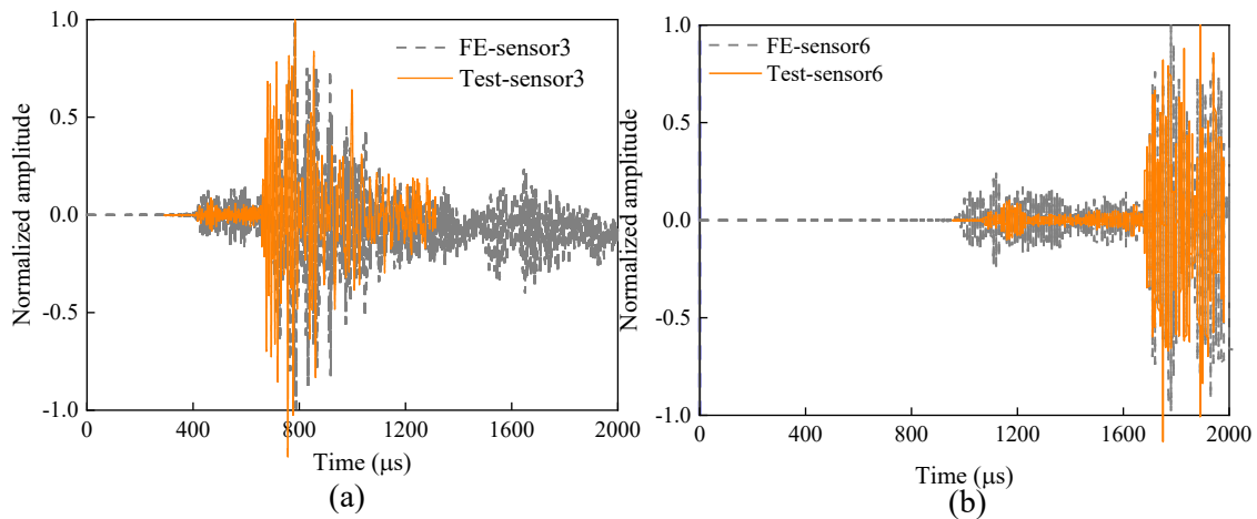
Fig. 6: Experimental vs. numerical received signal of (a) sensor 3 and (b) sensor 6 at linear array excited from E1
