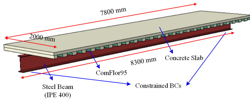
Fig. 1: Dimension of the composite steel-concrete girder
