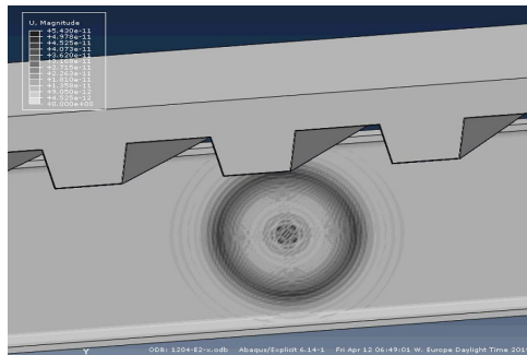
Fig. 5: Illustration of Lamb waves propagation in ABAQUS
