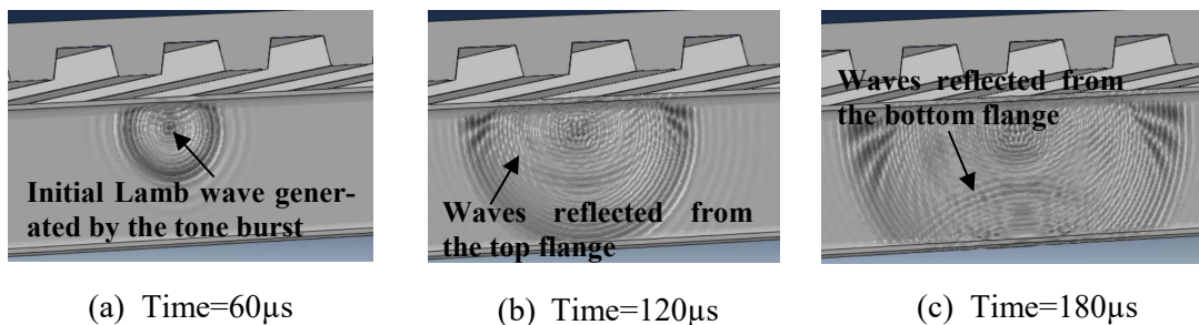
Fig. 12: Simulation of Lamb wave propagation in the girder
