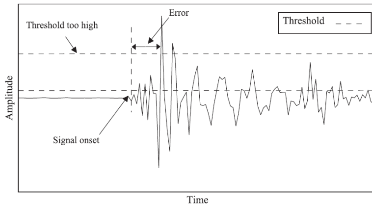
Fig. 7: Potential errors using the fixed threshold value method [7]
