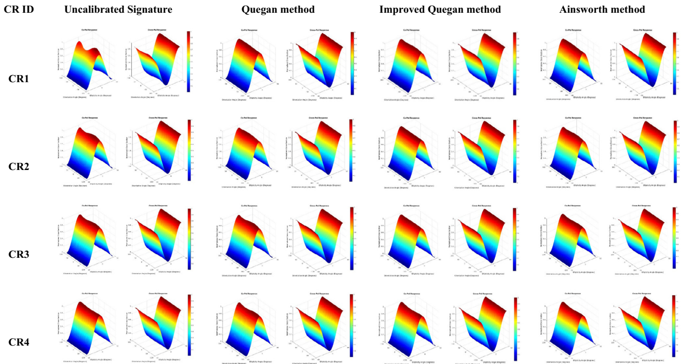
Fig. 10. Polarimetric Signatures of Trihedral corner reflectors extracted from 18-February-2019 RADARSAT-2 dataset.
