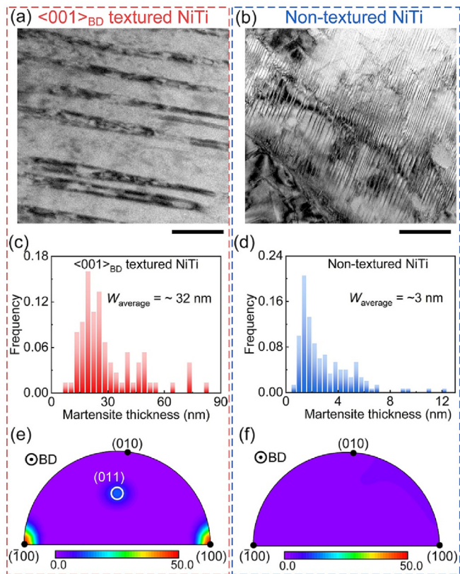
Fig. 11. Bright-field TEM images of (a, c) <001> BD textured and (b, d) non-textured AM NiTi samples, showing martensite size and morphology, and corresponding martensite width statistics; Inverse pole figures of B19' martensite phase measured by XRD in (e) <001> BD textured and (f) non-textured AM NiTi samples measured at RT; All scale bars are 100 nm.
