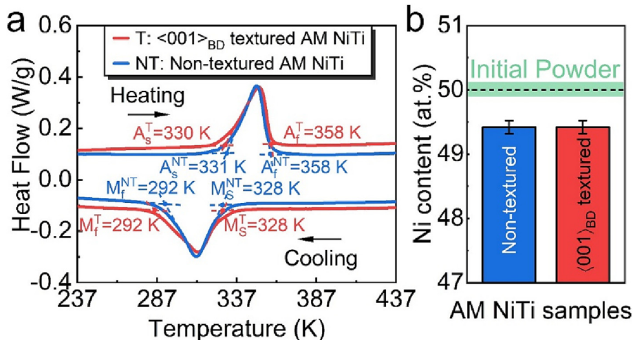
Fig. 8. (a) Differential scanning calorimetry (DSC) of as-fabricated \langle 001 \rangle_{BD} textured and non-textured AM NiTi; where, martensite start temperature is denoted as M_s , martensite finish temperature as M_f , austenite start temperature as A_s , and austenite finish temperature as A_f . (b) Ni content of \langle 001 \rangle_{BD} textured and non-textured AM NiTi samples measured by inductively coupled plasma-optical emission spectrometry (ICP-OES) with 0.1 at.% accuracy. T is \langle 001 \rangle_{BD} texture and NT is non-texture.
