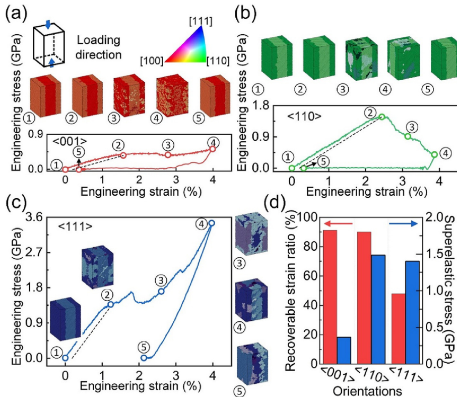
Fig. 4. MD simulations of 4% engineering strain compressive deformation of bicrystal NiTi periodic boundary conditions at 353 K, showing the behavior of (a) (001), (b) \langle 110 \rangle and (c) \langle 111 \rangle orientations; Corresponding simulated microstructures at different deformation stages are shown above the simulated stress–strain curves: ① the starting state, ② the critical point for stress-induced martensite transformation, ③ the intermediate state between ② and ④, ④ the position with 4% strain, and ⑤ the unloading state; the 0.2% strain offset method was used to identify critical stress for the stress-induced martensite transformation and different color domains within the simulated microstructures indicate grains with different orientations and martensite variants. (d) The recoverable strain ratios and superelastic stresses of various oriented models.
