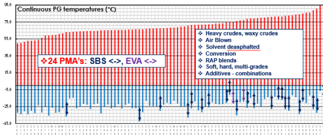
AIRC Binder Matrix - Performance Grade Mapping (°C)
