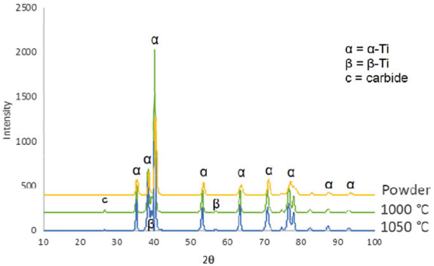
Fig. 4.13 XRD patterns of sintered \text{Ti}_6\text{Al}_4\text{V} and as-received powder
