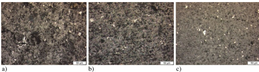
Fig. 4.9 Optical microscopy images of EAC-1A sintered samples with a 100 \mu m maximum particle size; b 50 \mu m maximum particle size; c 22 \mu m maximum particle size
