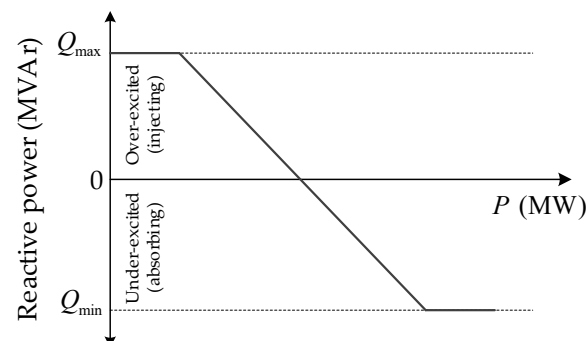
Figure 1. Smart inverter control based on Q(P) -characteristic.
