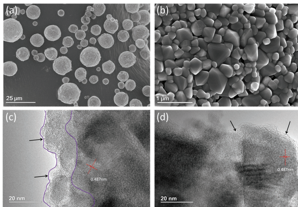
Figure 1. Morphology and structure of the spherical \text{Li}_4\text{Ti}_5\text{O}_{12} materials: a) SEM image of the pristine sample; b) magnified SEM image of the pristine sample; HR-TEM image of c) pristine sample and d) modified sample ( 0.008 \text{ mol L}^{-1} \text{ Na}_2\text{S} aqueous solution, 180^\circ\text{C} , 8 h).
