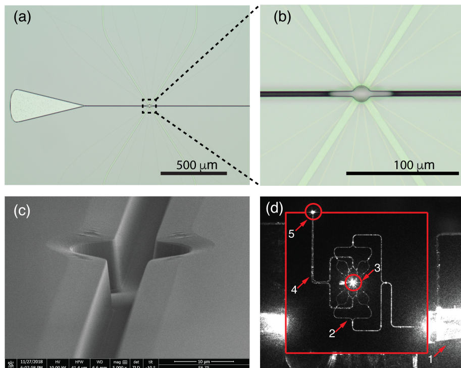
Figure 6: (a) Optical microscope image of a device with 16 excitation and 4 detection waveguides. (b) Magnification of the marked area in (a), clearly showing the 16 excitation waveguides and the 4 detection waveguides. (c) Scanning electron microscope image of the device, showing the 15 \mu\text{m} diameter central microbath with the 5 \mu\text{m} wide side channels. (d) Camera image of the 16-waveguide device actuated with light from the input fiber, which is embedded in a fiber array unit (FAU). The various structures light up as a result of light scattering, giving bright saturation of the camera. The red square indicates the chip edges. 1: FAU. The large saturation region results from scattering loss at the input waveguide. 2: Excitation-waveguide circuitry. 3: Microbath with the central trapping region. 4: Detection-waveguide circuitry. 5: Bright spot resulting from scattering of 785 nm light, coupled out from the multimode waveguide connected to the detection waveguides. The detection waveguides collect this light from the microbath at their facets, as a result of direct illumination and scattering.
