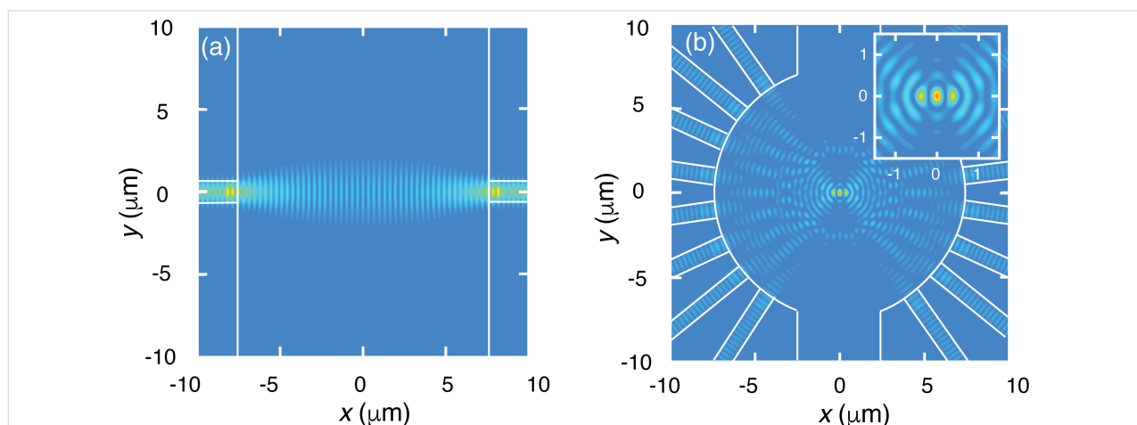
Figure 4: Energy density of the electric field in the multi-waveguide devices used in experimental demonstrations in this work. (a) 2-waveguide device with a 15 \mu\text{m} wide fluidic channel. (b) 16-waveguide device with a 15 \mu\text{m} diameter microbath and 5 \mu\text{m} wide side channels. The waveguides and the walls of the fluidic structures are indicated by white lines. For (a) and (b) the color scale indicating the energy density is the same.
