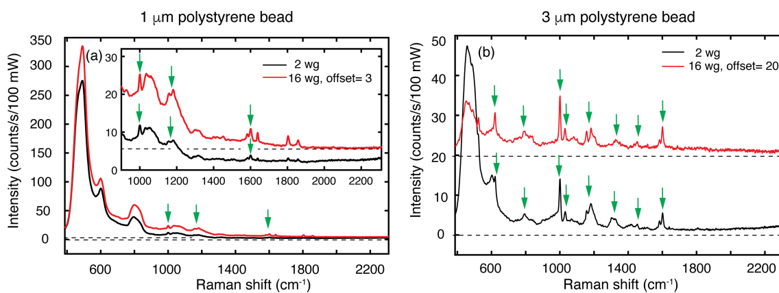
Figure 9: Raman spectra obtained with the 2-waveguide (black line) and the 16-waveguide (red line) trap for polystyrene beads with diameters of 1 and 3 \mu\text{m} . For the spectra obtained with the 16-waveguide trap, vertical offsets were applied as indicated in the legend. Each spectrum has its own horizontal axis drawn as a dashed black line. Identified characteristic Raman peaks of polystyrene are denoted by arrows. In (a) the inset is a magnification of a part of the main plot.
