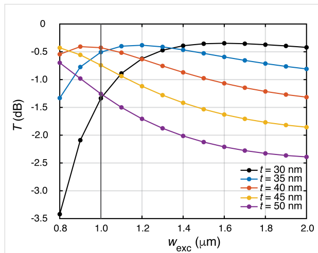
Figure 3: Fiber-to-chip transmission T as a function of the waveguide width w_{\text{exc}} for various thicknesses t . The vertical line indicates the chosen waveguide width.
