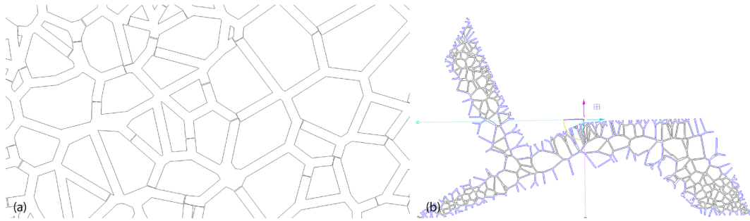
FIGURE 4 Conversion of cellular geometry (a) into robotic toolpaths (b).
