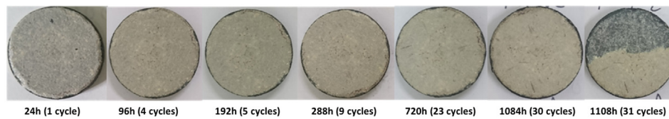
Fig. 6. Evolution of damaging during thermal cycling at 1100 °C of a complete self-healing TBC system made by spark plasma sintering of a mixture of YPSZ powder and 10 vol% encapsulated MoSi 2 (B) based particles sintered on a NiCrAlY coated substrate.
