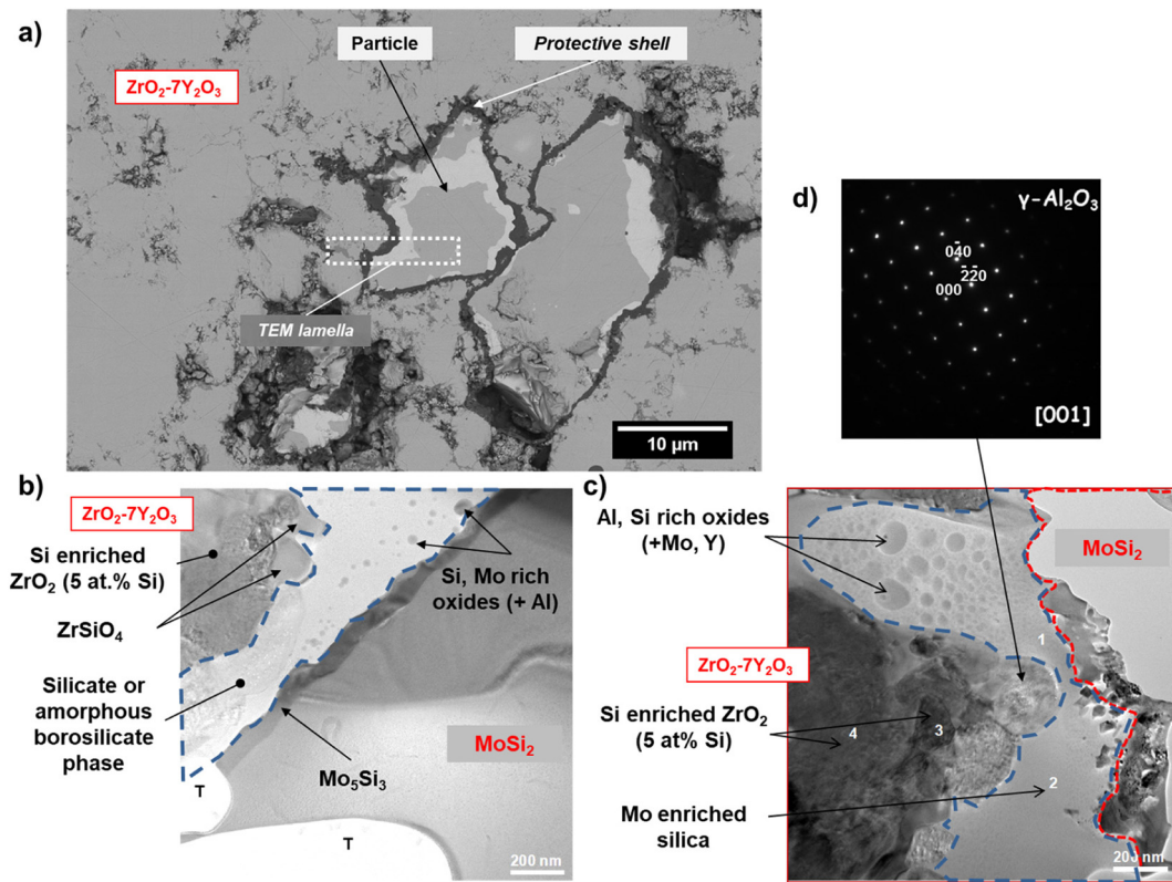
Fig. 3. Composite of encapsulated MoSi 2 (B) based healing particles embedded in YPSZ after annealing in Ar at 1100 °C for 24 h: (a) cross-section of the composite just before lift-out of a thin FIB lamella. (b) and (c) TEM images of the FIB lamella after final thinning. (d) diffraction pattern of a \gamma -Al 2 O 3 crystallite. Here, 'T' denotes some undesirable pores introduced during the thinning process.
