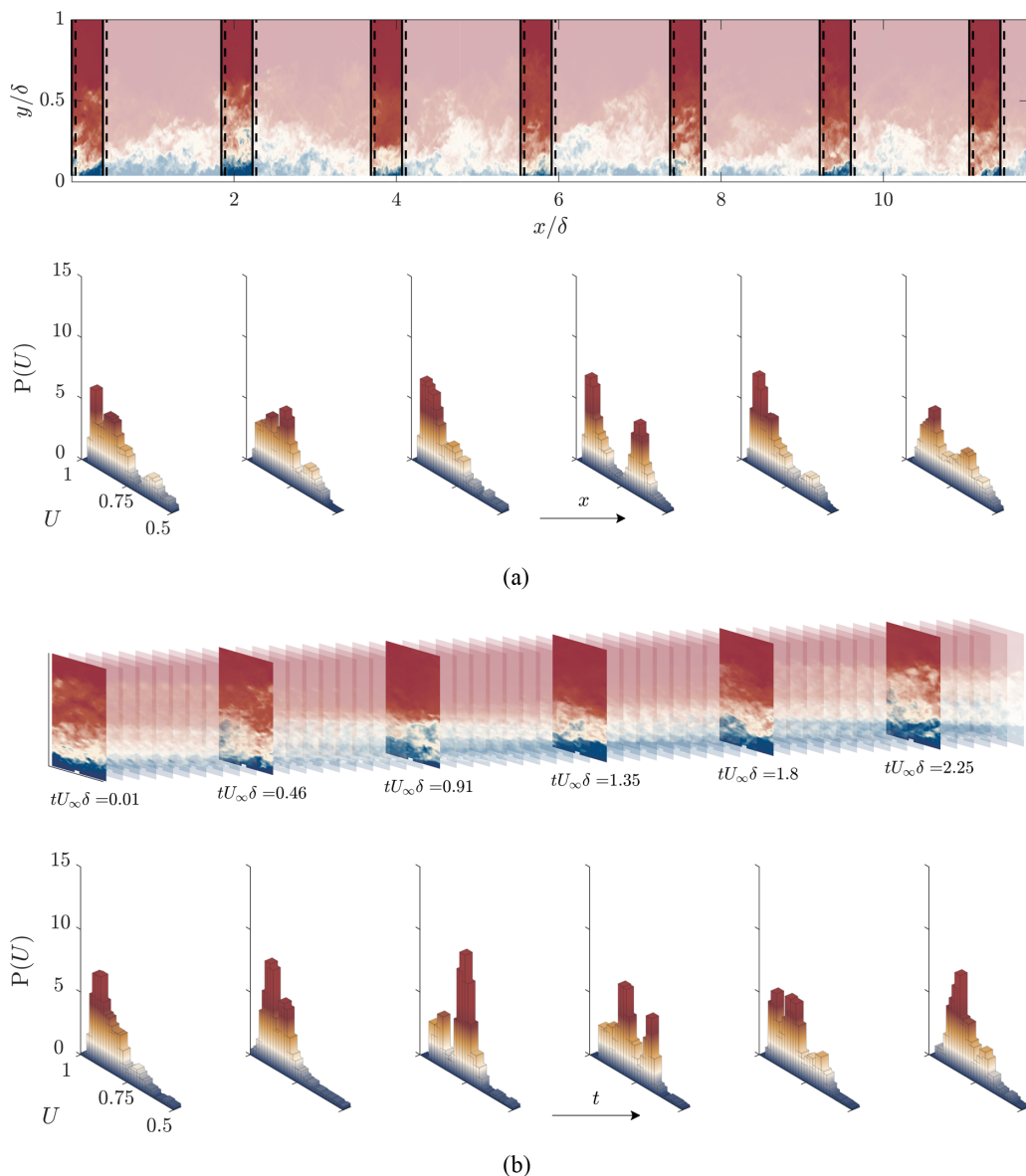
FIG. 1. Construction of \mathcal{P}(U, t) : (a) Spatial data (SPIV1, SPIV2, SPIV3, SPIV4, AEM), (b) temporal data (TRPIV, R1, R2). In (a), the full spatial extent, L_x , is divided into regions of L_x^+ |_{\text{PDF}} = 2000 , while the same extent is selected from the time-resolved snapshots in (b). To match the temporal resolution in (b), an appropriate level of spatial overlap is used for each consecutive region in (a) (indicated with dashed lines) when constructing the PDF, while also assuming a constant U_c = 0.81 .
