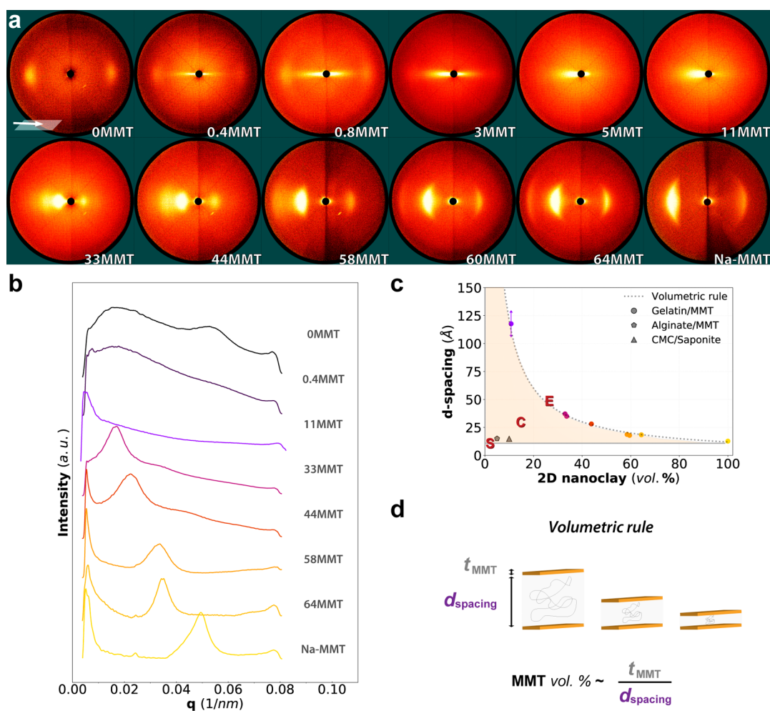
Figure 2. (a) 2D transmission X-ray scattering images of gelatin/MMT samples with varying volumetric MMT composite contents at beam inclination parallel to the plane of the films (90.5–94° range of glancing angle). The scattering patterns reveal anisotropy and a progressive change in basal reflections with increasing clay loadings. (b) Wide-angle X-ray diffractograms depict a peak shift of d_{001} MMT reflections toward higher angles starting from sample 11MMT. (c) Comparison between experimental and calculated d -spacings derived from the d_{001} MMT reflection. The thickness of a delaminated Na-MMT platelet was obtained by reciprocal fit of d_{001} lengths and extrapolating to origin (virtual zero concentration). Alginate and carboxymethyl cellulose composite data, respectively, from Zlopasa et al. 30 and Ebina and Mizukami. 18 (d) Illustration depicting the theoretical basis for calculating d -spacing, where a reciprocal volumetric rule of concentration of MMT is assumed; t_{\text{MMT}} is the thickness of a single platelet, and d_{\text{spacing}} is the platelet interspace.
