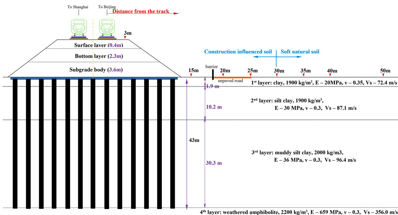
Fig. 2. Schematic diagram of the cross section and measurement points at various distances from the track (E – Young’s modulus, ν – Poisson’s ratio, Vs – shear wave velocity).
