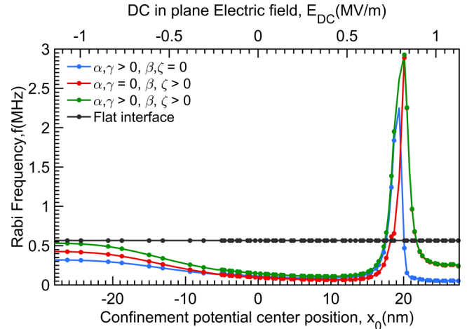
FIG. 4. EDSR Rabi frequency f_{\text{Rabi},v-} as a function of the quantum dot potential center position x_0 in a global magnetic field B = 1T along [001] with a step height of 5.43 \text{ \AA} . The enhancement appears at x_0 = 20 \text{ nm} , on the right side of the step.
