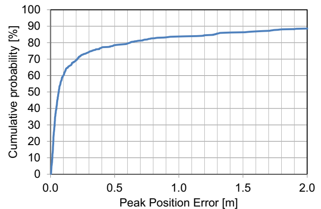
Fig. 8 Cumulative distribution of peak overlap errors in the CASSIOPE orbit determination
