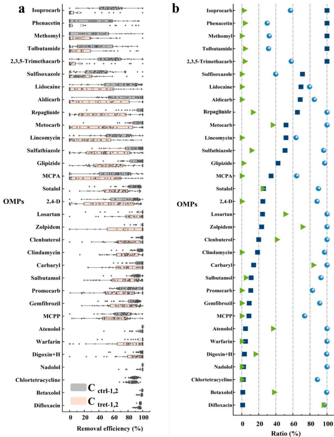
Fig. 3. (a) Thirty-two OMPs with significantly lower removal efficiency in C_{tret-1,2} than in C_{ctrl-1,2} . (b) ● The median of removal efficiencies in the column study ( C_{ctrl-1,2} ). ■ The inhibition ratio of OMP removal efficiency by the addition of ATU. ► OMP removal efficiency merely through sand adsorption in batch tests.
