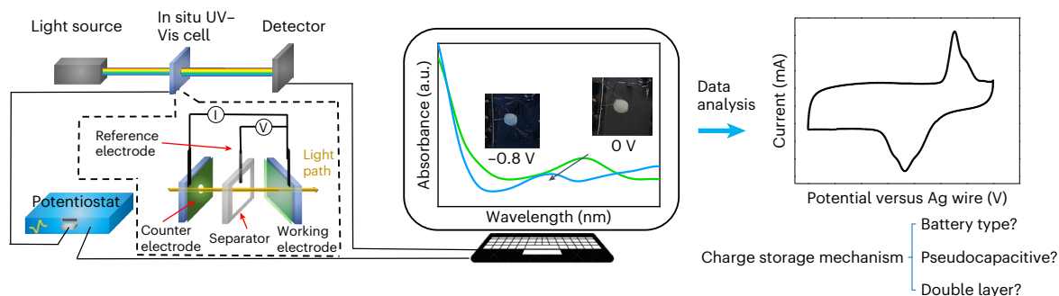
Fig. 1 The setup for in situ electrochemical UV-Vis spectroscopy. A simple three-electrode in situ UV-Vis cell is designed to allow electrochemical characterization with simultaneous recording of UV-Vis absorption spectra. Analysis of the UV-Vis data allows one to distinguish intercalation-based battery-
