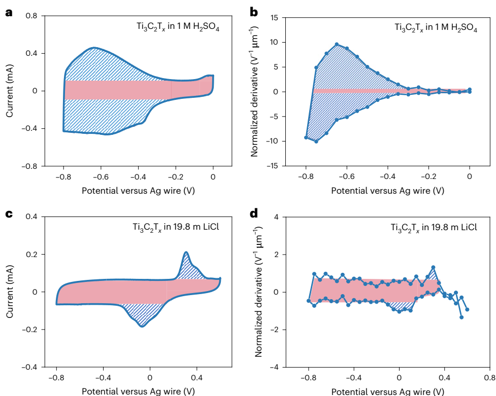
Fig. 5 | EDL and surface redox contributions to the total charge for \text{Ti}_3\text{C}_2\text{T}_x in different electrolytes. a, c, CV curves at 20 \text{ mV s}^{-1} for \text{Ti}_3\text{C}_2\text{T}_x in 1 \text{ M H}_2\text{SO}_4 (a) and \text{Ti}_3\text{C}_2\text{T}_x in 19.8 \text{ m LiCl} (c). b, d, Normalized derivative versus potential collected
