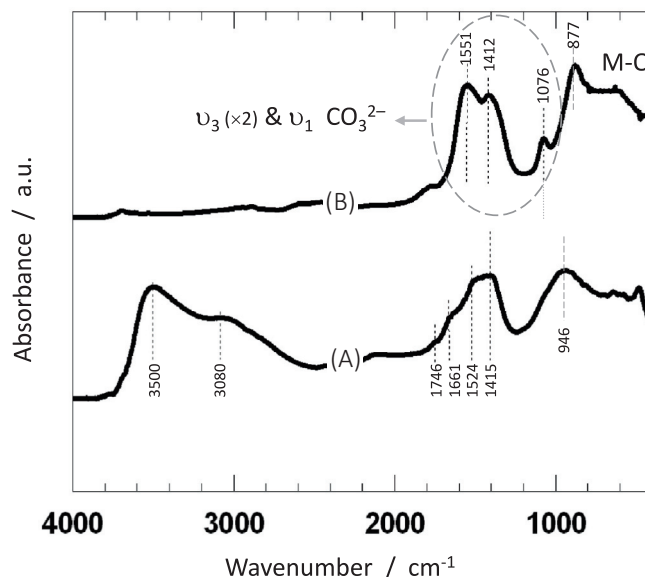
Fig. 2. In situ DRIFT spectra of the as-synthesized hydrotalcite, dried at 100^\circ\text{C} (A) and after synthetic air treatment at 350^\circ\text{C} (B).
