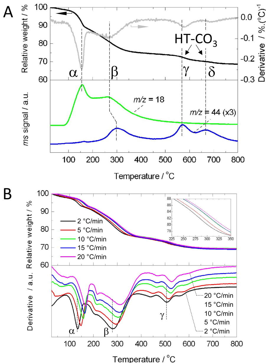
Fig. 3. A) Thermal decomposition of the Cu-Zn-Al hydrotalcite in synthetic air: top ) TGA and DTGA profiles; bottom ) EGA profiles for H 2 O ( m/z = 18 ) and CO 2 ( m/z = 44 ) fragments. B) Top ) TGA and bottom ) DTGA patterns for the Cu-Zn-Al hydrotalcite decomposition in air at different heating rates used to derive data for the model fittings in Fig. 4. The inset in the top graph represents the amplification of the 225–350 °C region to show the trend; the shift into higher temperatures due to the heating rate's increase.
