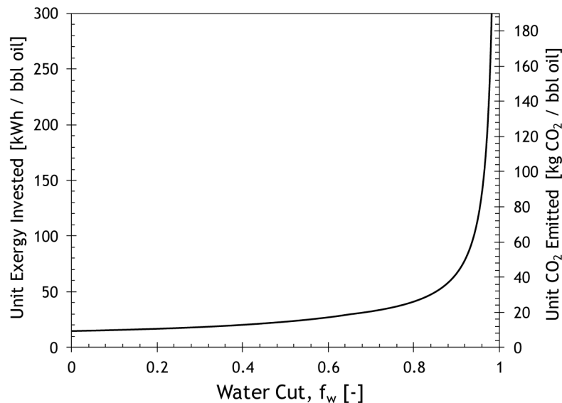
Figure 3—Unit exergy consumed and CO 2 emitted as functions of water cut for the water-injection case.
