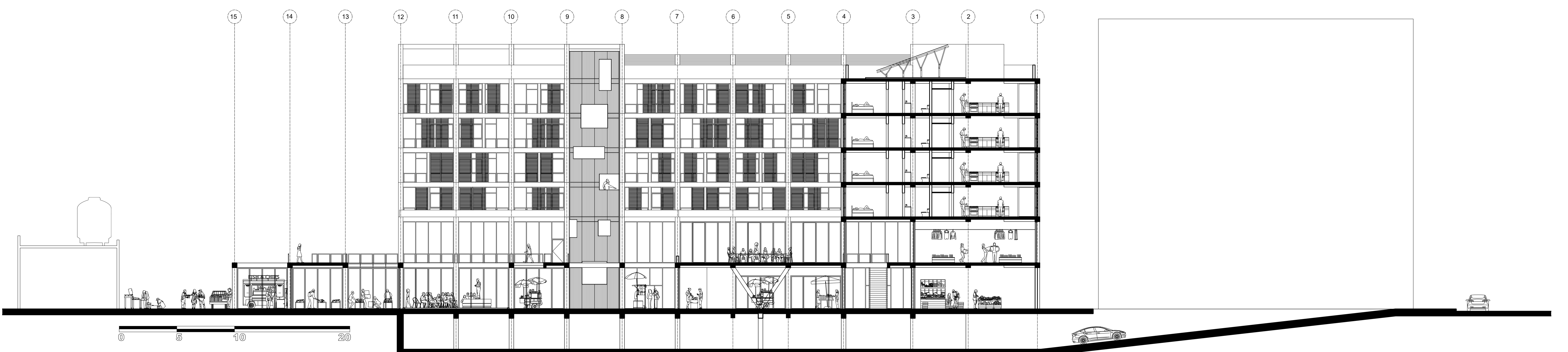
F-F' Section Scale 1/200
