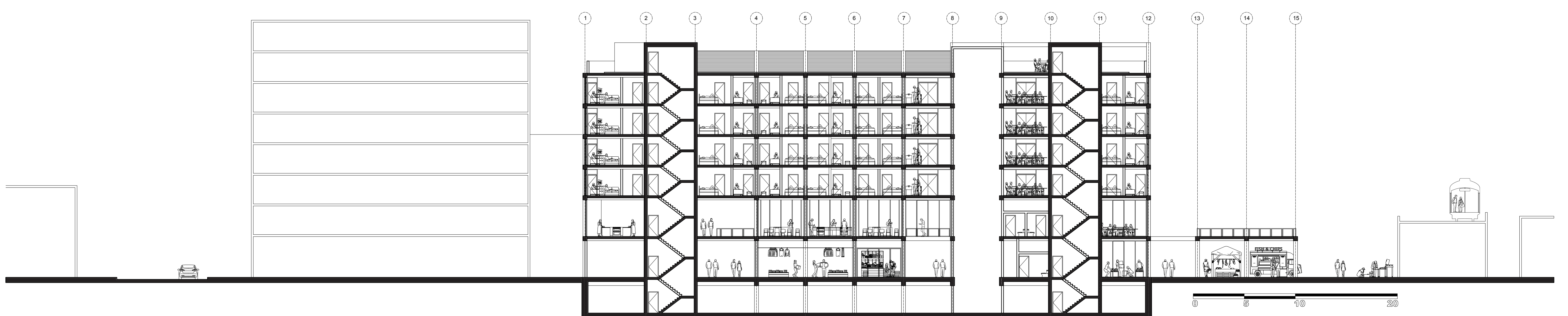
C-C' Section Scale 1/200
