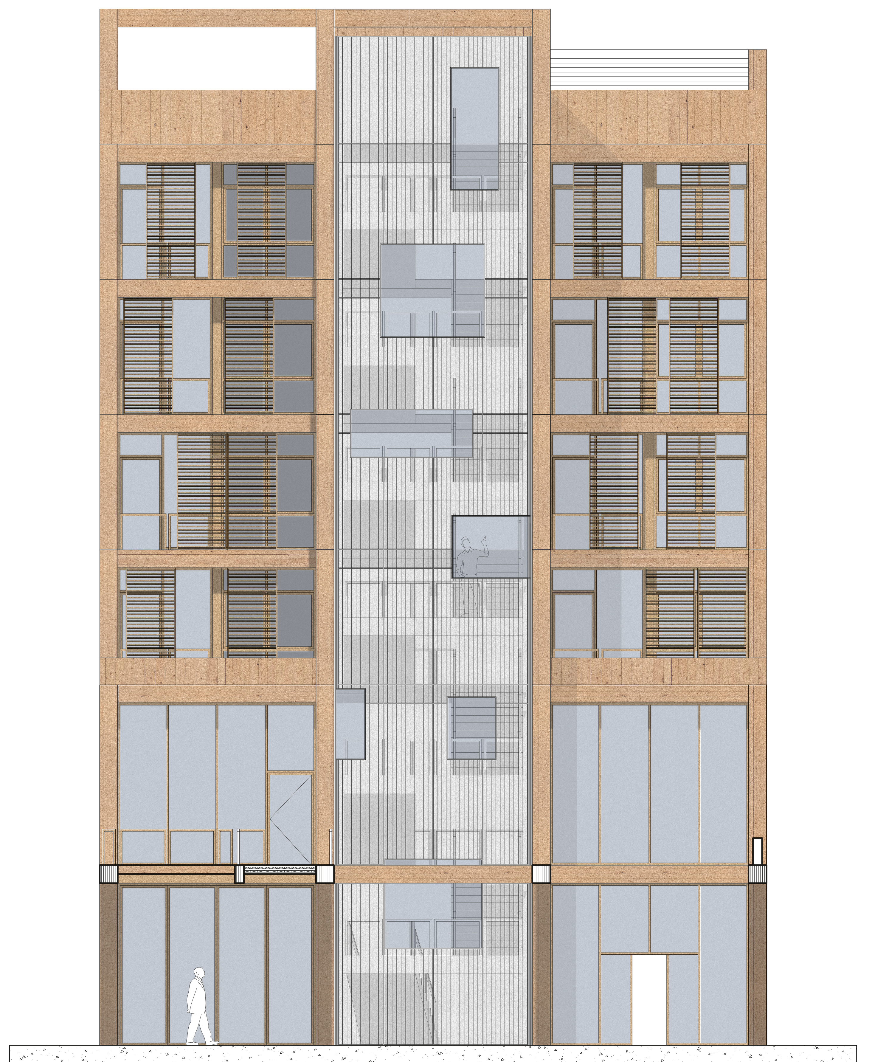
Fragment Elevation East Facade Scale 1/50
