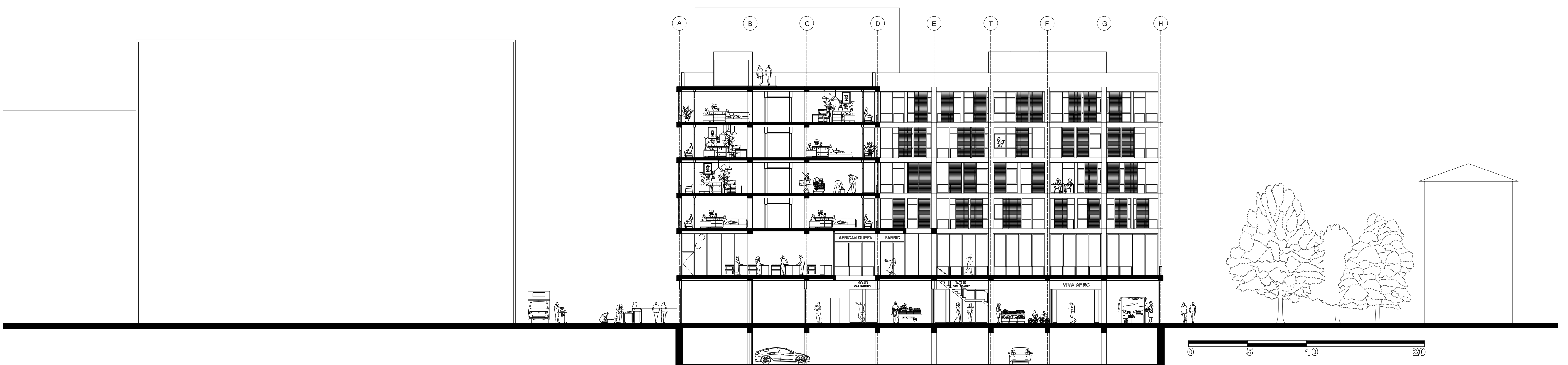
A-A' Section Scale 1/200
