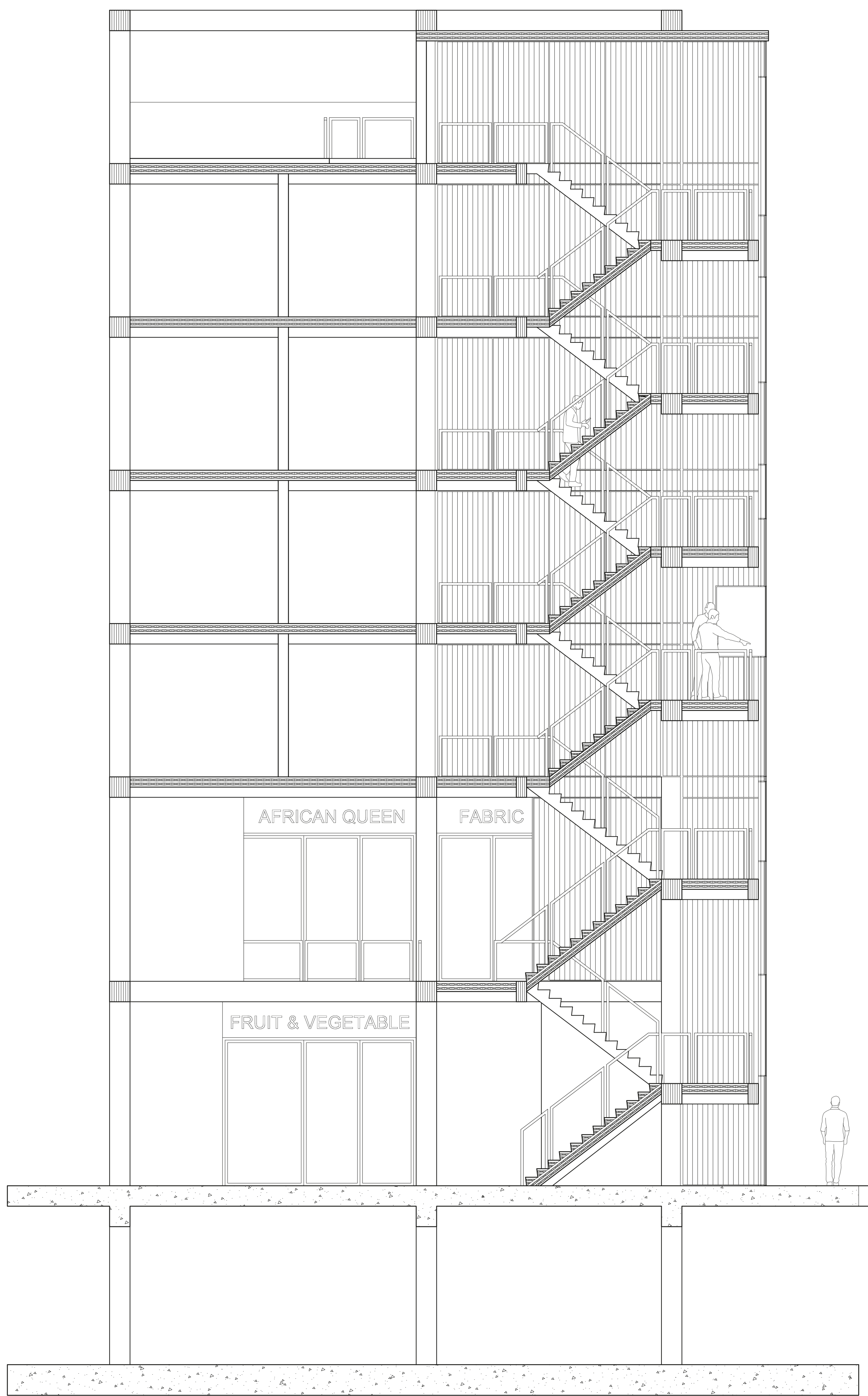
Fragment Section Scale 1/50
