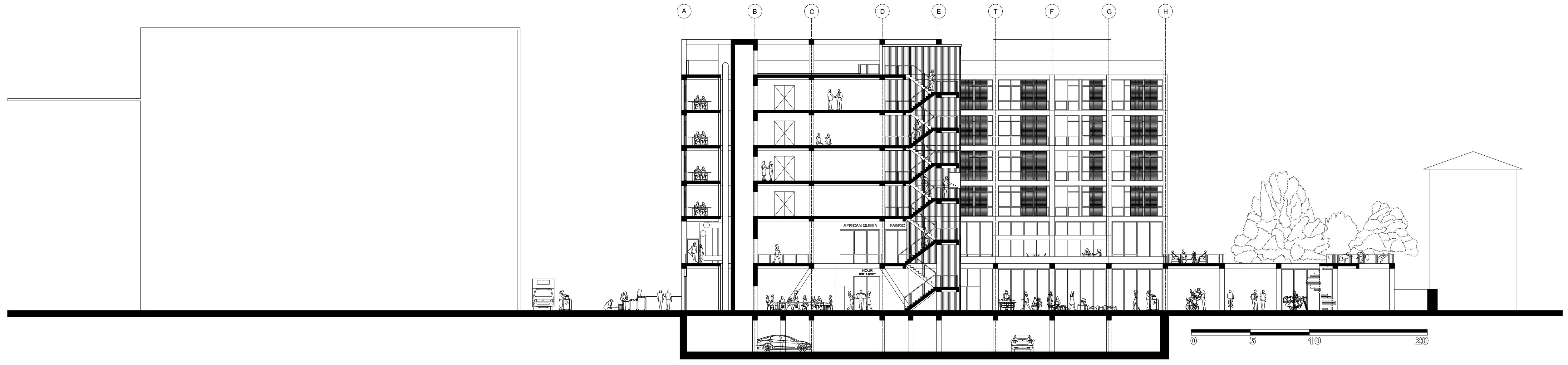
E-E' Section Scale 1/200
