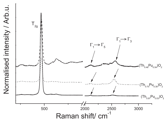
Fig. 4. Raman spectra recorded with a 647-nm excitation source mixed ThO_2 - PuO_2 oxides. The spectra are truncated between 900\text{ cm}^{-1} and 2000\text{ cm}^{-1} for a better readability.
