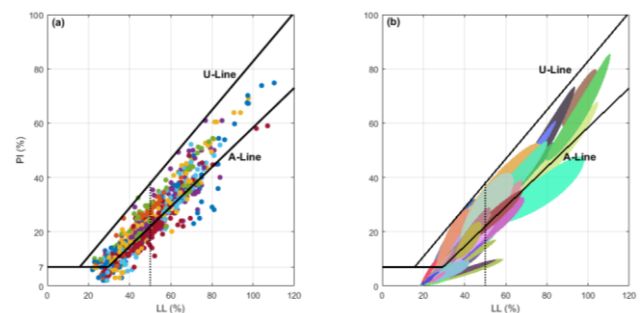
Figure 7. (a) (LL, PI) data; (b) cross-correlations of the hypothetical sites generated by the trained HBM.
