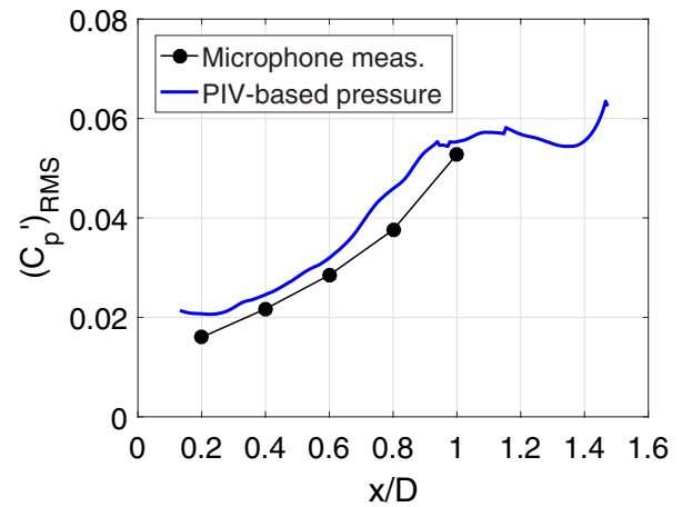
Figure 28. RMS of pressure fluctuations on the afterbody.
