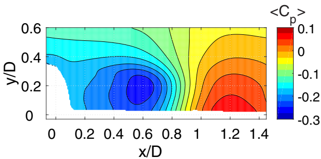
Figure 25. Mean pressure.
