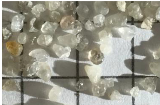
Fig. 2. Rapid sand filter granules 0.8 < d_p < 1.25 mm.
