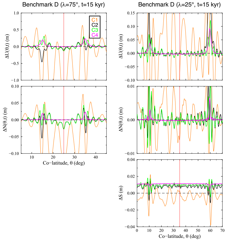
Figure A1. The differences arising from the VEGA C i solutions, i = 1, \dots, 4 , with respect to VEGA ref along the co-litudinal cross-sections shown in the right panels of Figs 14 (left) and 15 (right) for benchmark D. The four combinations C1,...,C4 of the input parameters for the VEGA C i solutions are given in Table A1.
