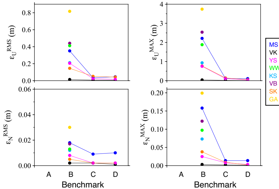
Figure 21. The same as Fig. 20, but for the co-latitude cross-sections through the centre of the ocean basin, which are shown in the left-hand panels of Figs 6, 10 and 15 for benchmark examples B–D. The results for benchmark A are not applicable since an ocean basin is not considered in this case.
