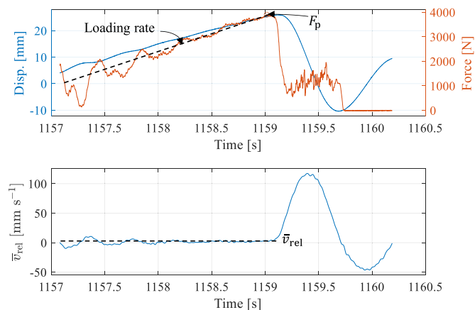
Fig. 18. Single cycle of IC, experimental data from base case test ID 410.
