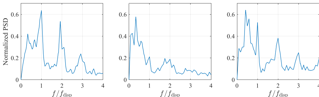
Fig. 17. Normalized and summed PSDs of ice forces during the first 12 cycles of FLI, measured forces (left) against simulated forces with only a positive force-velocity gradient (middle) and simulated forces with a positive and negative force-velocity gradient (right).
