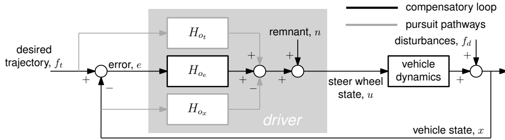
Figure 1: Driver-vehicle control diagram that illustrates the possible driver responses, based on [McR67]. The single-loop compensatory control organization is shown in black, while additional pursuit pathways are shown in gray. The driver's possible (proprioceptive) pursuit response on the steering wheel state u is not shown, because it is not considered in this paper.
