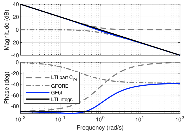
Fig. 3. Magnitude- and phase-characteristics of LTI element C_{PI} ( \omega_c = 1 ), the SIDF of a GFORE ( \gamma = 0 ) with \omega_r as in (8), and the SIDF of their series connection, compared with LTI integrator C_{int} .
