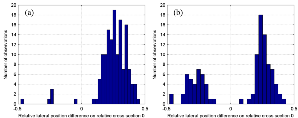
Figure 3.10: Histograms of relative lateral position difference of overtaken and overtaking vessels at relative cross section 0 in Sea-Nieuwe Maas (a) and Nieuwe Maas-Sea (b).
