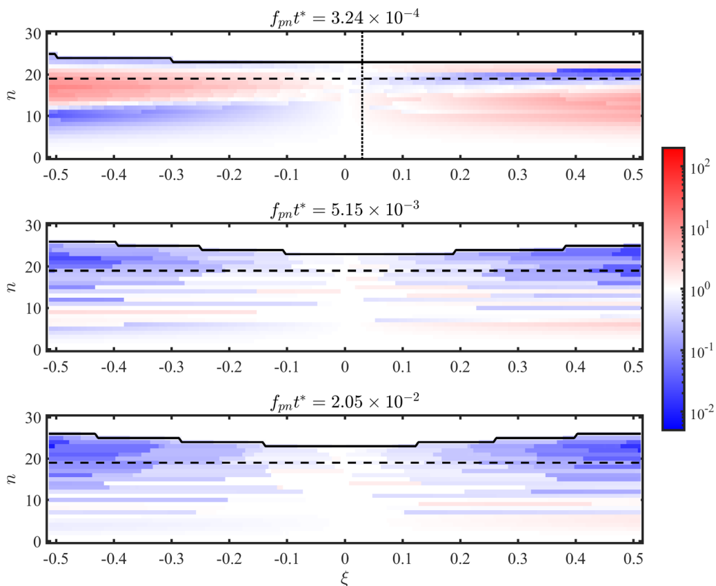
FIG. 9. The same plots as Fig. 3, but shown for a sinusoidal flow rate with an additional sinusoidal peristaltic waveform Q_p \sin(2\pi f_{per}t) added about the mean flow rate for all cases considered. A constant Q_p = 0.486Q_0 based on the magnitude of the first peristaltic harmonic is set for the CFR case in Fig. 8(b). Using this value, the oscillatory parameter is limited to \xi \leq 0.51 to maintain a positive injection rate. The \xi -axis and color ( \epsilon -axis) limits in this plot differ from those in Fig. 3.
