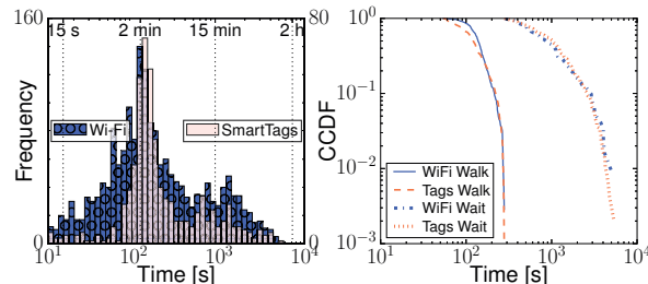
Fig. 6: Crowd Flow [Left] Time between vantage points. [Right] Estimated walking and waiting times between vantage points.
