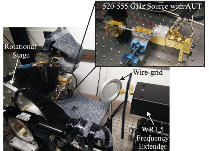
Fig. 6: Photograph of the antenna far-field measurement setup with a 520-555 GHz source with our antenna under test (AUT) mounted on two rotational stages. A WR1.5 frequency extender is used as a receiver.
