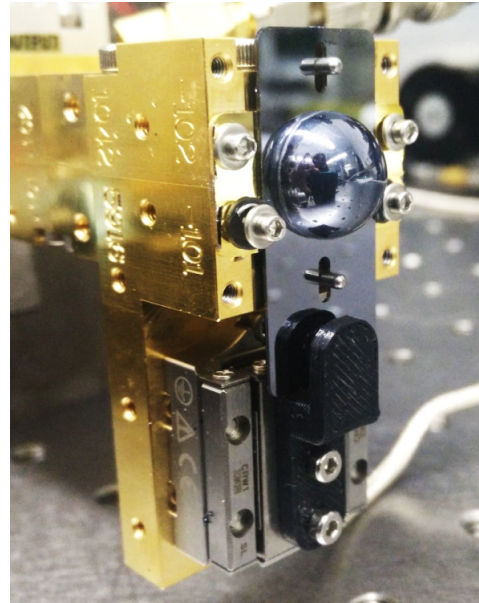
Fig. 1: Photograph of the prototype at 550 GHz of the silicon lens fed by a leaky-wave waveguide feed with an integrated piezo-electric motor. The hemispherical silicon lens has a radius of 6 mm.
