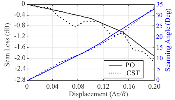
Fig. 4: (Left Axis) Scan loss and (Right Axis) scanning angle as a function of the lens displacement of the lens-antenna for L = 0.04R .
