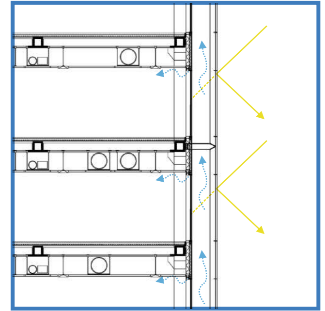
Triple solar glazing Ventilated facade
