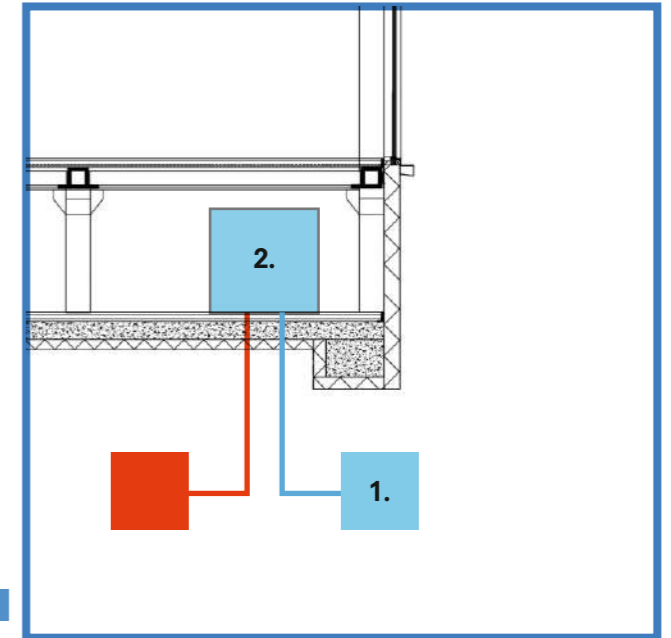
1. Geothermal energy storage 2. Heat pumps for heating and cooling
