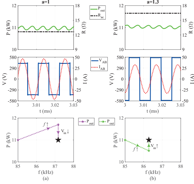
Fig. 3. Operating circuit waveforms of the 11 kW S-S compensation network in Fig. 2 with ZVS turn-on ( f > f_0 ), where: (a) a=1 , (b) a=1.3 .
