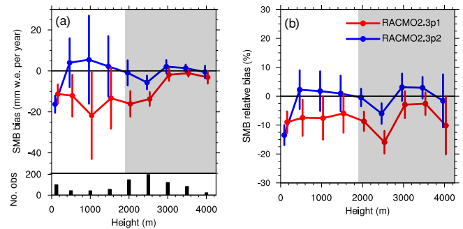
Figure 8. (a) Absolute bias and (b) relative bias ((model – observation)/model \times 100 %) in modelled SMB for RACMO2.3p2 (blue) and RACMO2.3p1 (red). The data are binned in 500 m surface elevation intervals (0–250, 250–750, etc.). Error bars denote the combined uncertainty of the model and observations within each height bin, based on Van de Berg et al. (2006) and Van Wessem et al. (2014a). Elevations above 2000 m (shaded grey) represent East Antarctica exclusively. The bar chart in (a) denotes the number of weighted observations in each bin. To separate blue and red lines, x axis locations of each bin are displaced by 75 m.
