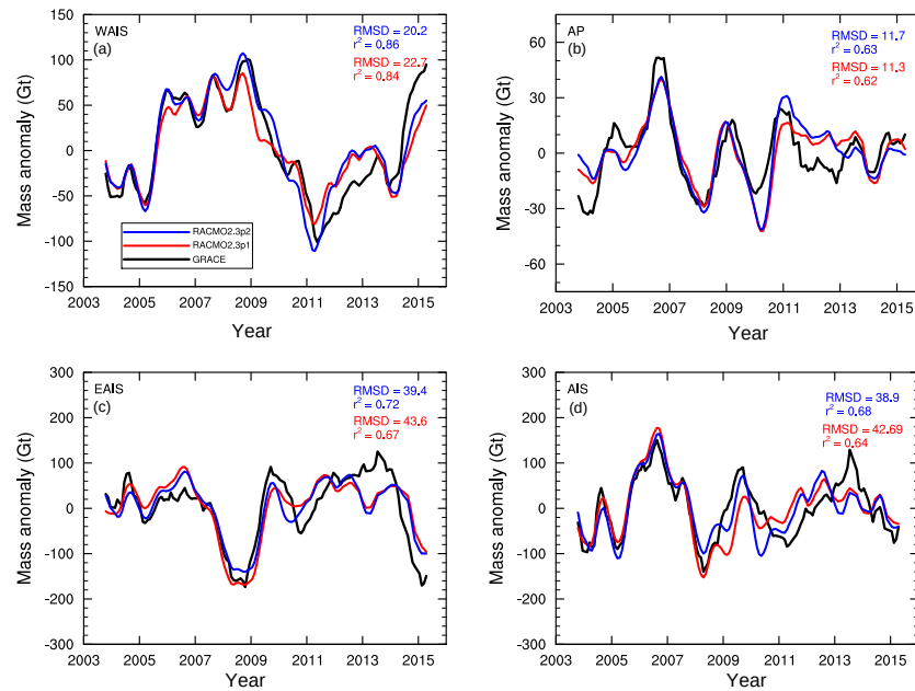
Figure 9. Detrended and decelerated average (for details see text) SMB anomalies of RACMO2.3p2 (blue), RACMO2.3p1 (red) and GRACE (black) release RL05 for West Antarctica (a), the Antarctic Peninsula (b), East Antarctica (c) and the whole Antarctic ice sheet (AIS, d). Shown are root mean square deviation (RMSD) and correlation ( r^2 ).
