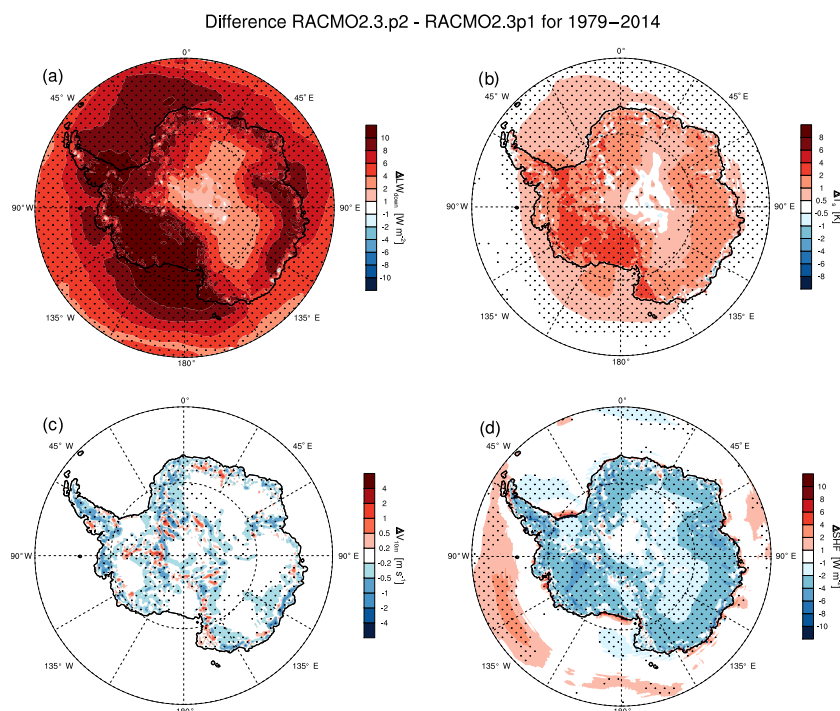
Figure 2. Annual average (1979–2014) difference (RACMO2.3p2–RACMO2.3p1) of (a) downwelling longwave radiation ( LW_d ), (b) surface temperature ( T_s ), (c) 10 m wind speed ( V_{10m} ) and (d) sensible heat flux (SHF). Areas where the difference exceeds 1 standard deviation of the difference are stippled.
