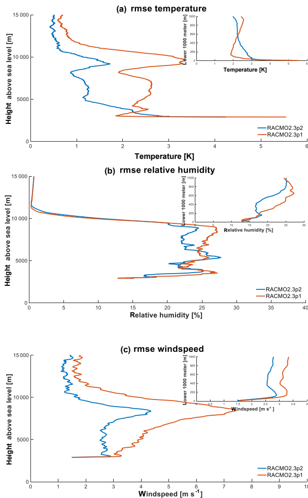
Figure 7. Root mean square error (RMSE) of average upper-atmosphere temperature (a), relative humidity (b) and wind speed (c) from RACMO2.3p2 (blue) RACMO2.3p1 (red) and the radiosonde observations at Kohnen Station, from January 2014. Note that the lowermost level is at the surface of Kohnen Station, at \sim 3000 m elevation. Subpanels show a close-up of the lower 1000 m.
