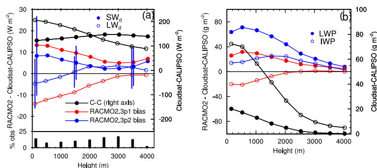
Figure 6. (a) Absolute bias (left axis) in average (2007–2010) modelled downwelling longwave radiation ( LW_d ) (open circles) and downwelling shortwave radiation ( SW_d ) (closed circles) and (b) cloud ice water path (IWP) (open circles) and cloud liquid water path (LWP) (closed circles) for RACMO2.3p2 (blue) and RACMO2.3p1 (red) compared to the CloudSat–CALIPSO product (Van Tricht et al., 2016b). Also shown on (a) and (b) are the observational data (black circles, right axis). Error bars in (a) denote the root mean square difference (RMSD) from a statistical comparison of the CloudSat–CALIPSO fluxes and ground-based AWS observations (Van Tricht et al., 2016a), only shown for three bins as based on the elevations of the four ground-based AWSs used. The data are binned in 500 m surface elevation intervals (0–250, 250–750, etc.). The bar chart in (a) denotes the percentage of total grid points per elevation bin. To separate LW_d and SW_d fluxes, x axis locations of each bin in (a) are displaced by 60 m.
