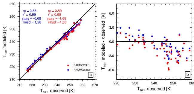
Figure 5. (a) RACMO2.3p2 (blue) and RACMO2.3p1 (red) and (b) modelled minus observed 10 m snow temperature as a function of the 10 m snow temperature observations. Denoted are the slope, determination coefficient r^2 , bias and root mean square deviation (RMSD) for both model versions.
