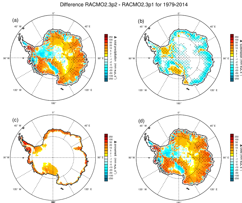
Figure 3. Annual average (1979–2014) difference (RACMO2.3p2–RACMO2.3p1) of (a) total precipitation (snow and rain), (b) total drifting snow and surface sublimation, (c) snowmelt and (d) SMB. Areas where the difference exceeds 1 standard deviation of the difference are stippled.
