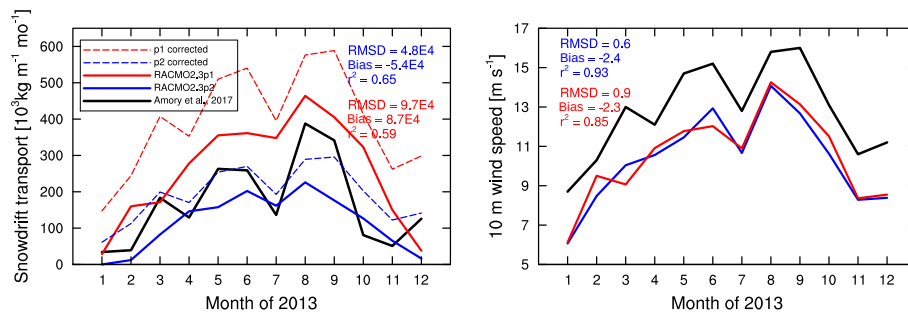
Figure 10. Monthly horizontal snow drift transport, TR_{ds} ( 10^3 \text{ kg m}^{-1} \text{ month}^{-1} ) (a), and 10 m wind speed, V_{10m} (b), from Amory et al. (2017), RACMO2.3p2 (blue) and RACMO2.3p1 (red) for the year 2013. The observed snow flux is calculated for the first 2 m only. The dashed lines represent the modelled transport fluxes corrected for the bias in V_{10m} , using a first-order linear regression.
