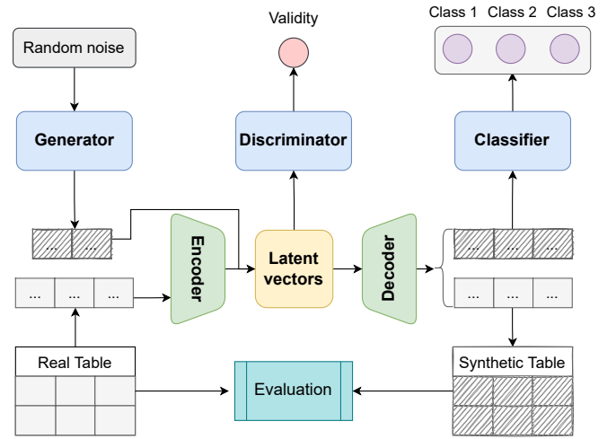
Fig. 3. The overall architecture and data flow of AE-GAN.
