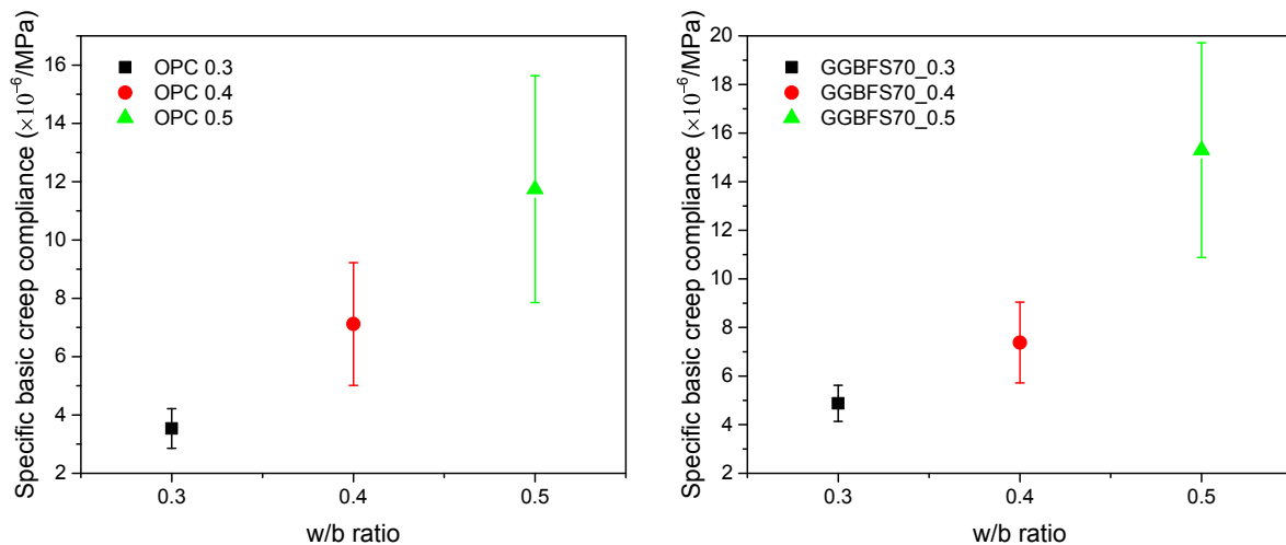
Fig. 10. The specific basic creep compliance measured at 800 s.
