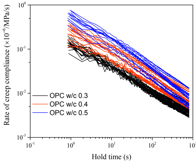
Fig. 12. The creep rate of cement pastes with different w/c ratios.
