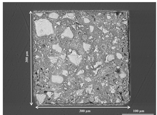
Fig. 2. ESEM image of the cross-sections of cantilever beam.
