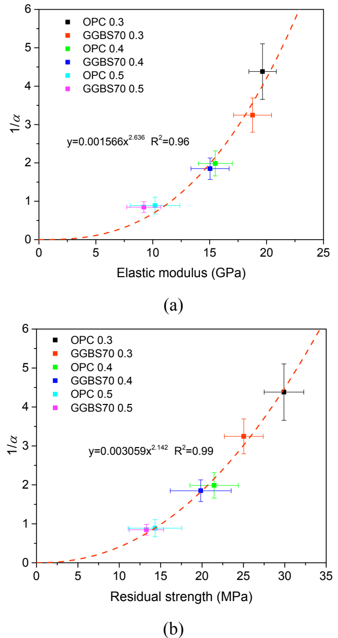
Fig. 14. The relationship between the inverse of \alpha and (a) the elastic modulus, and (b) the residual flexural strength.
