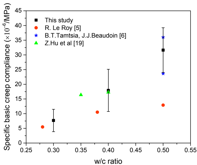
Fig. 16. The comparison with the specific basic creep compliance in macroscopic tests at 0.1 day.
