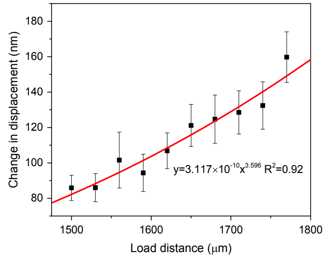
Fig. 9. The variation of change in displacement with different loading distance.
