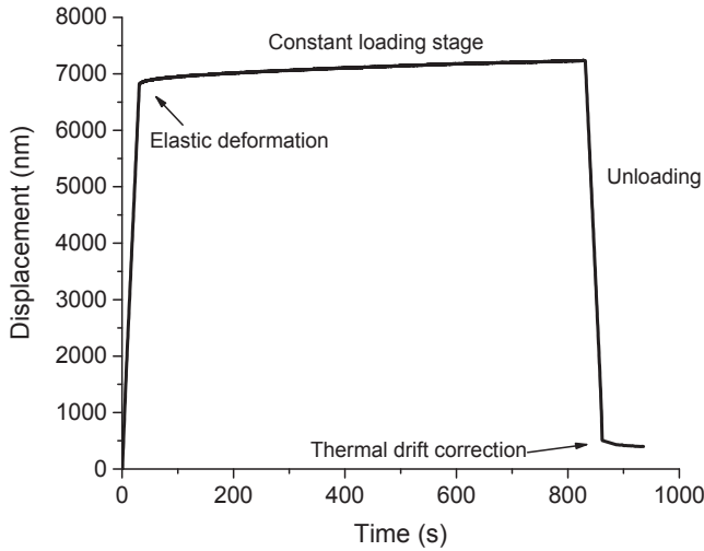
Fig. 7. Typical displacement-time curve for creep test.
