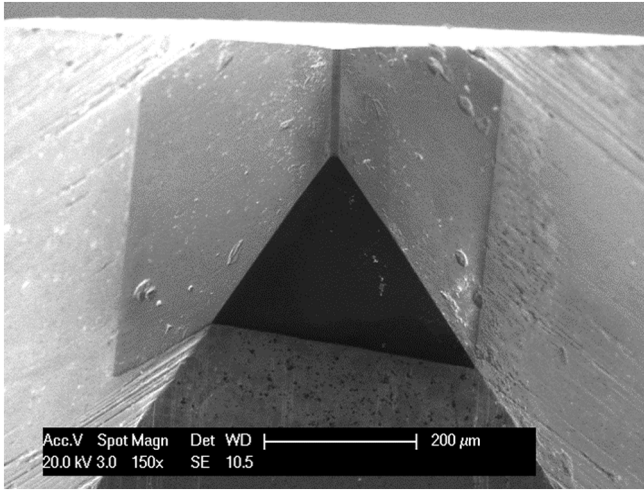
Fig. 3. ESEM micrograph of the diamond cylindrical wedge tip.
