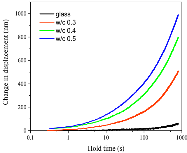
Fig. 8. Comparison of the change in displacement for glass and cement paste beams.
