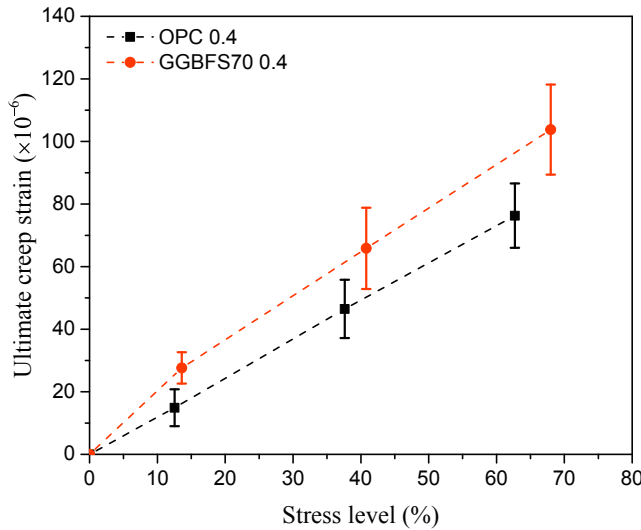
Fig. 13. The effect of stress level on ultimate creep strain at 800 s for two paste series with w/b of 0.4.
