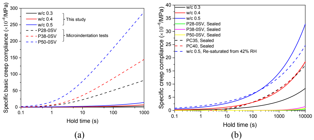
Fig. 15. The comparison with (a) microindentation tests [14] and (b) macroscopic tests [6,14,19]. The numbers after the ‘P’ or ‘PC’ represent the w/c ratio.
