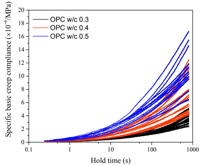
Fig. 11. The specific basic creep compliance with respect to the logarithmic time.
