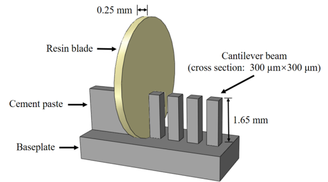
Fig. 1. Schematic diagram of sample preparation.
