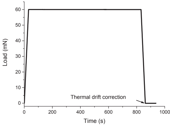
Fig. 6. Loading history of creep tests for w/c 0.3 OPC under the load level of 60mN.
